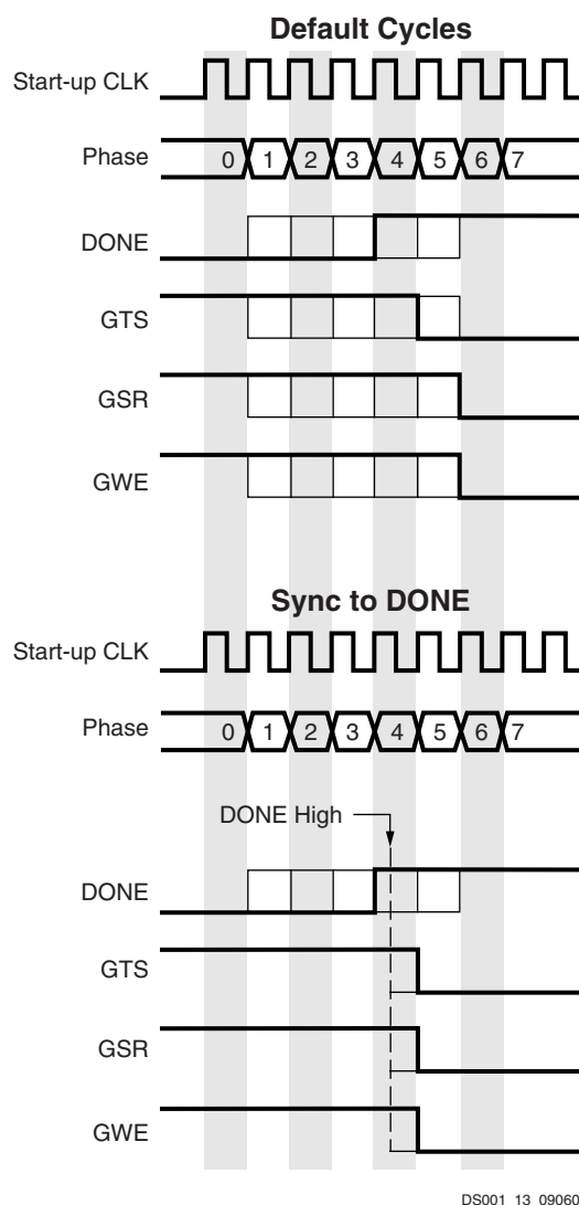
Figure 17: Start-Up Waveforms
