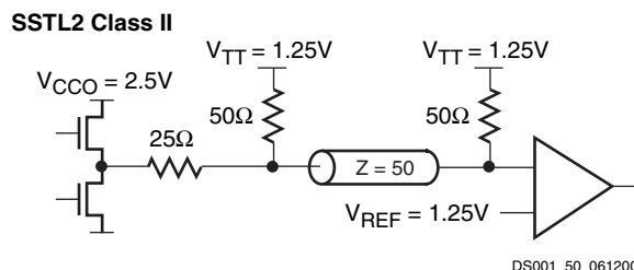
Figure 50: Terminated SSTL2 Class II
