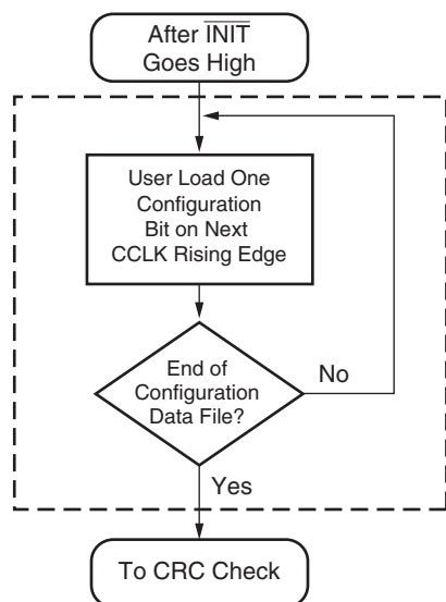
Figure 18: Loading Serial Mode Configuration Data
