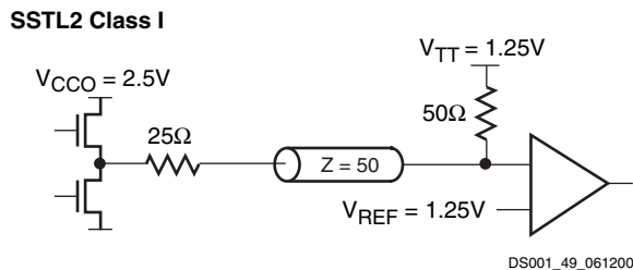
Figure 49: Terminated SSTL2 Class I
