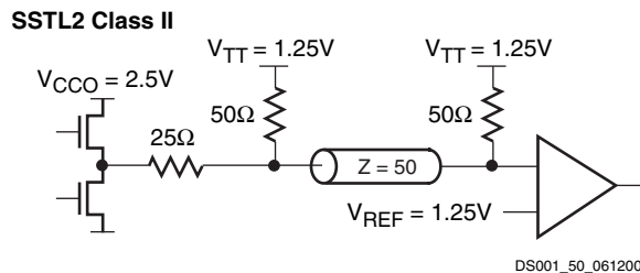
Figure 50: Terminated SSTL2 Class II
