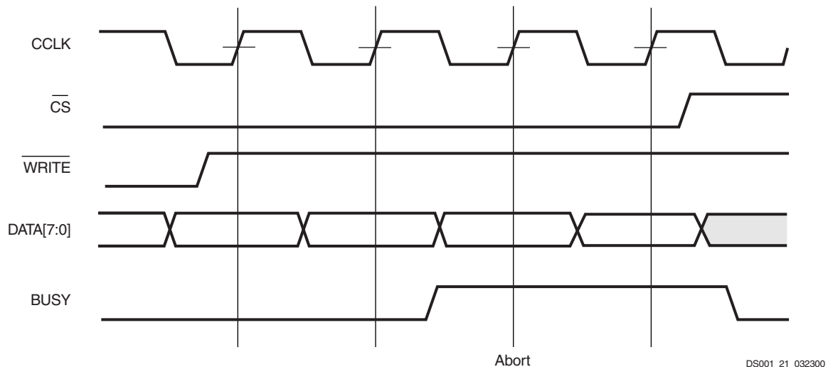
Figure 21: Slave Parallel Write Abort Waveforms
