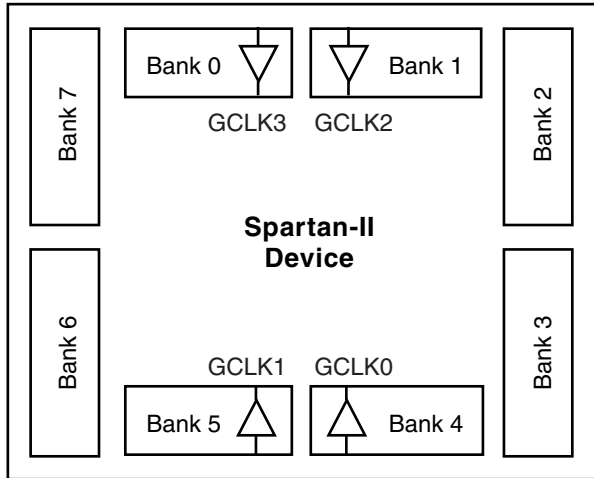
Figure 36: I/O Banks
