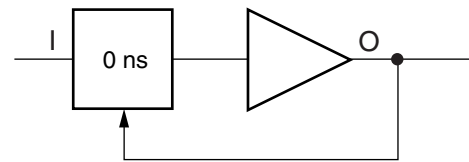
Figure 22: Simplified DLL Macro BUFGDLL
