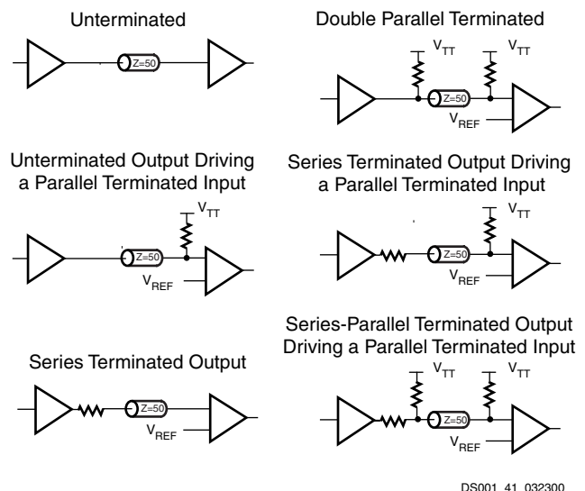
Figure 41: Overview of Standard Input and Output Termination Methods
