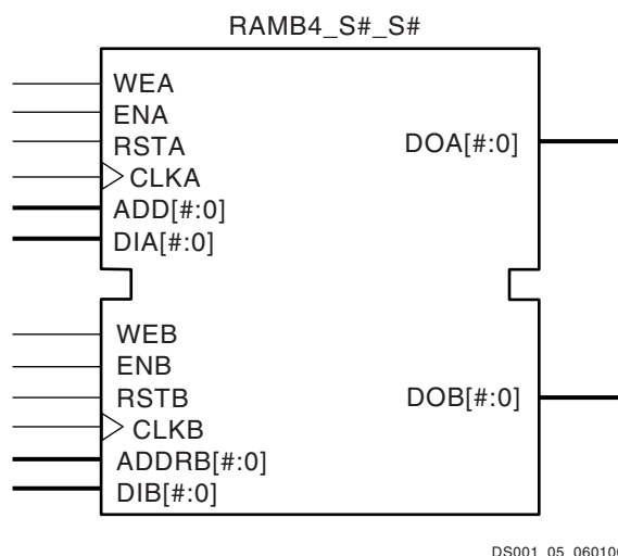
Figure 5: Dual-Port Block RAM
