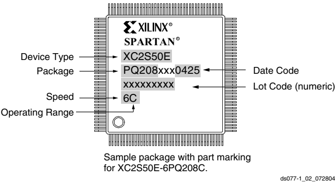
Figure 2: Spartan-IIE QFP Marking Example
