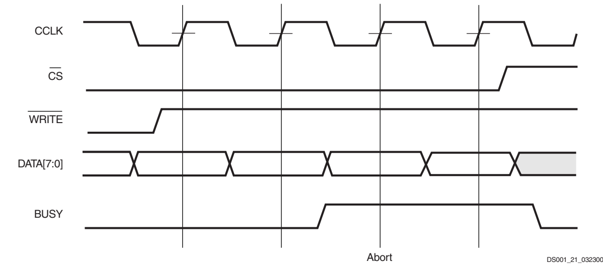
Figure 27: Slave Parallel (SelectMAP) Mode Write Abort Waveforms
