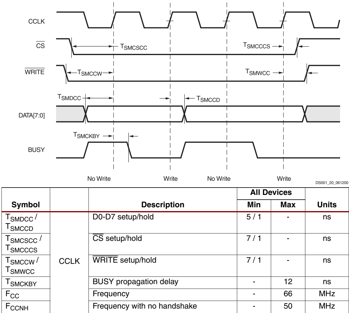
Figure 26: Slave Parallel (SelectMAP) Mode Write Timing
