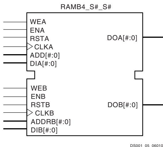
Figure 8: Dual-Port Block RAM
