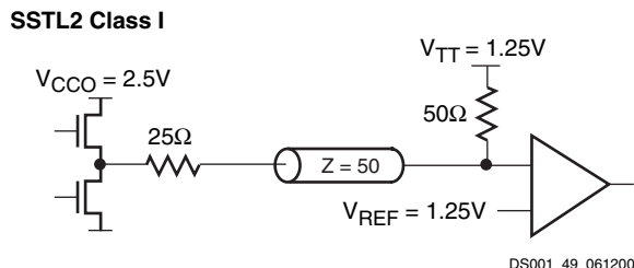
Figure 49: Terminated SSTL2 Class I
