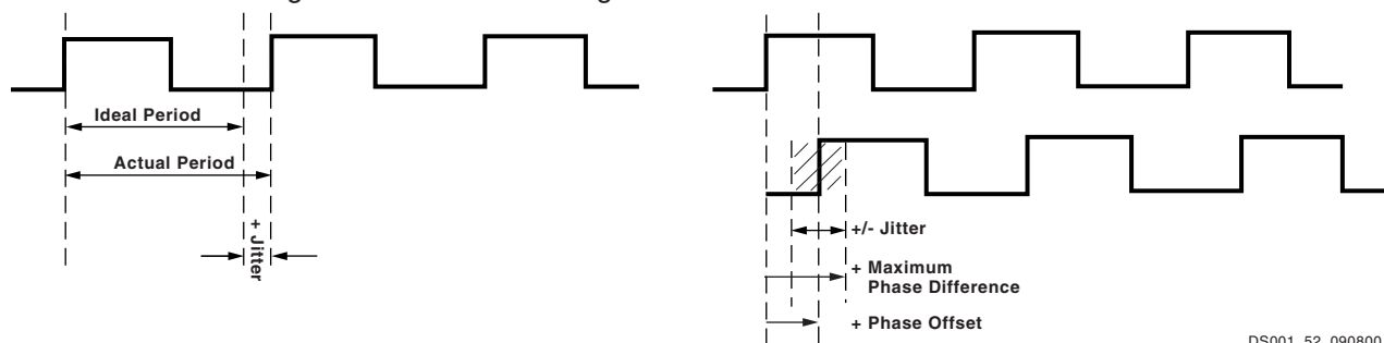
Figure 22: Period Tolerance and Clock Jitter
