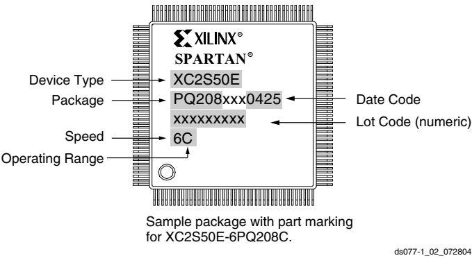
Figure 2: Spartan-IIE QFP Marking Example
