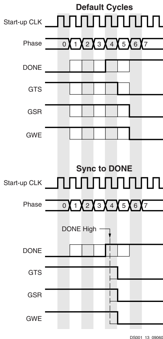
Figure 17: Start-Up Waveforms
