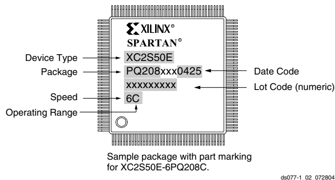
Figure 2: Spartan-II QFP Marking Example
