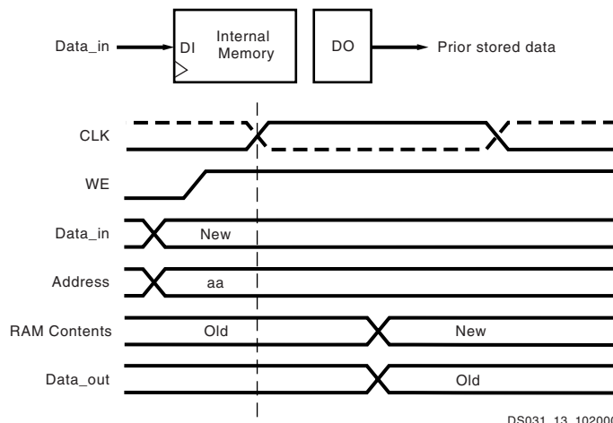
Figure 32: READ_FIRST Mode
