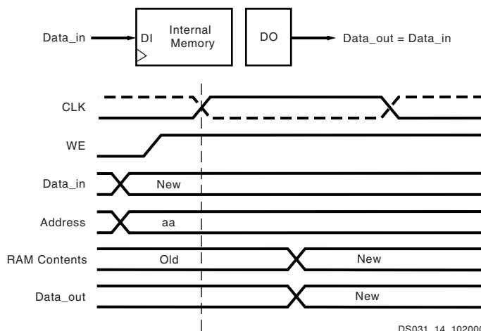
Figure 31: WRITE_FIRST Mode
