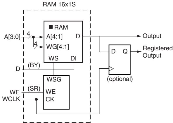
Figure 18: Distributed SelectRAM (RAM16x1S)
