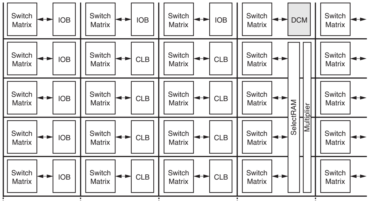
Figure 48: Routing Resources
