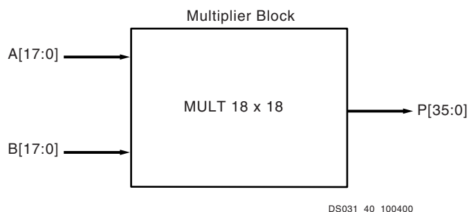
Figure 36: Multiplier Block
