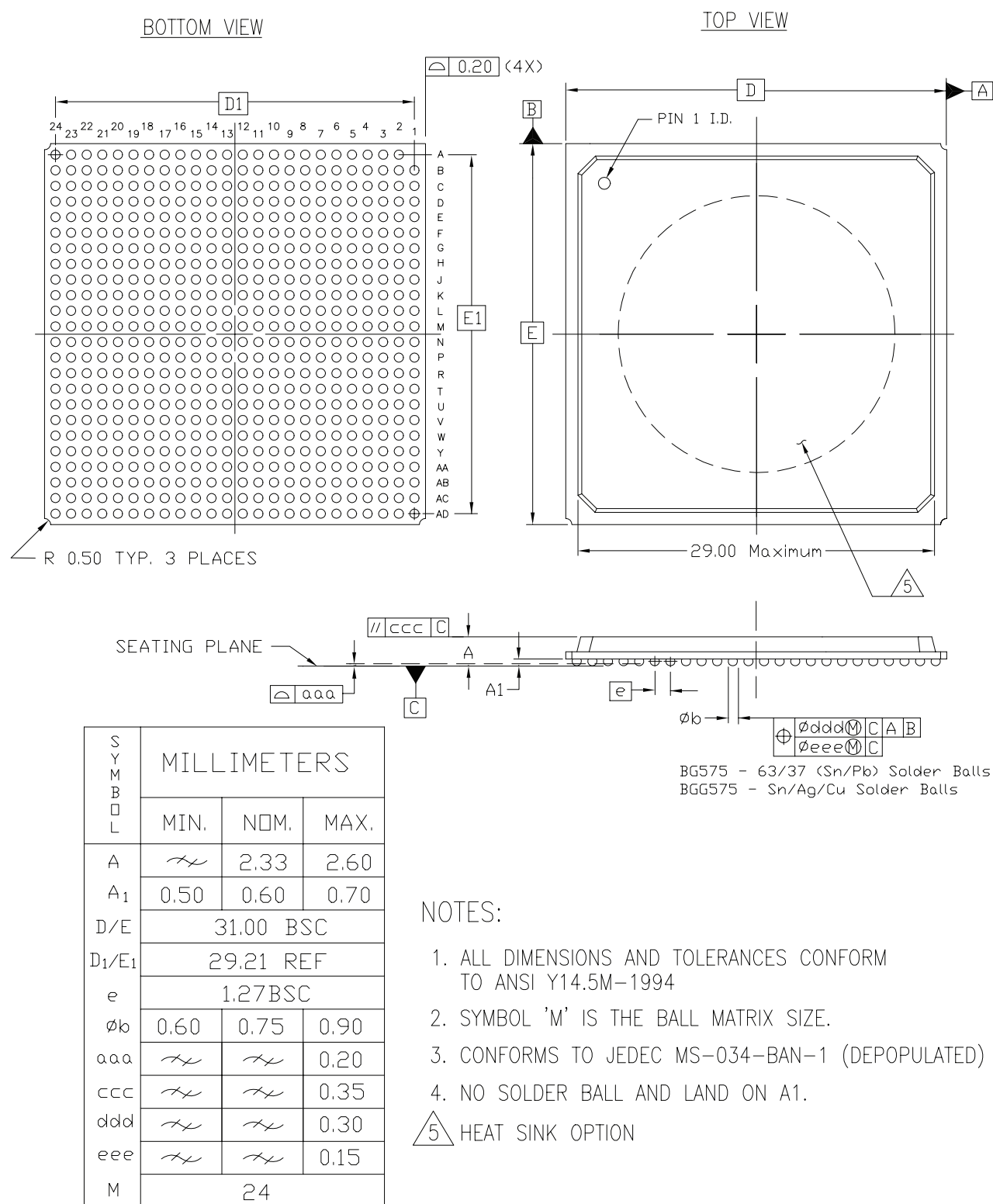
575-BALL MOLDED BGA (BG575/BGG575)
