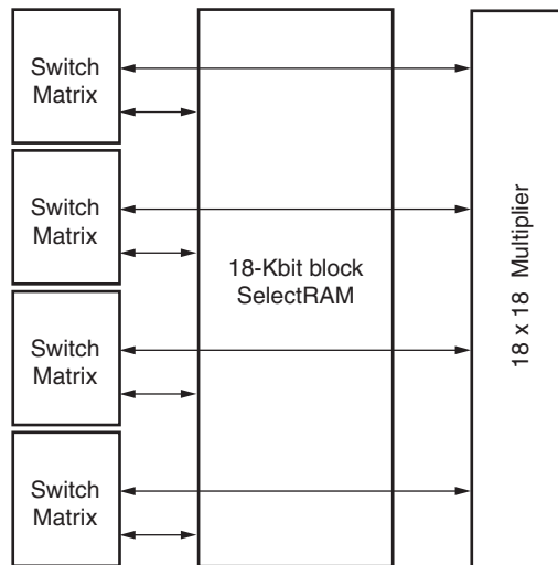
Figure 35: SelectRAM and Multiplier Blocks
