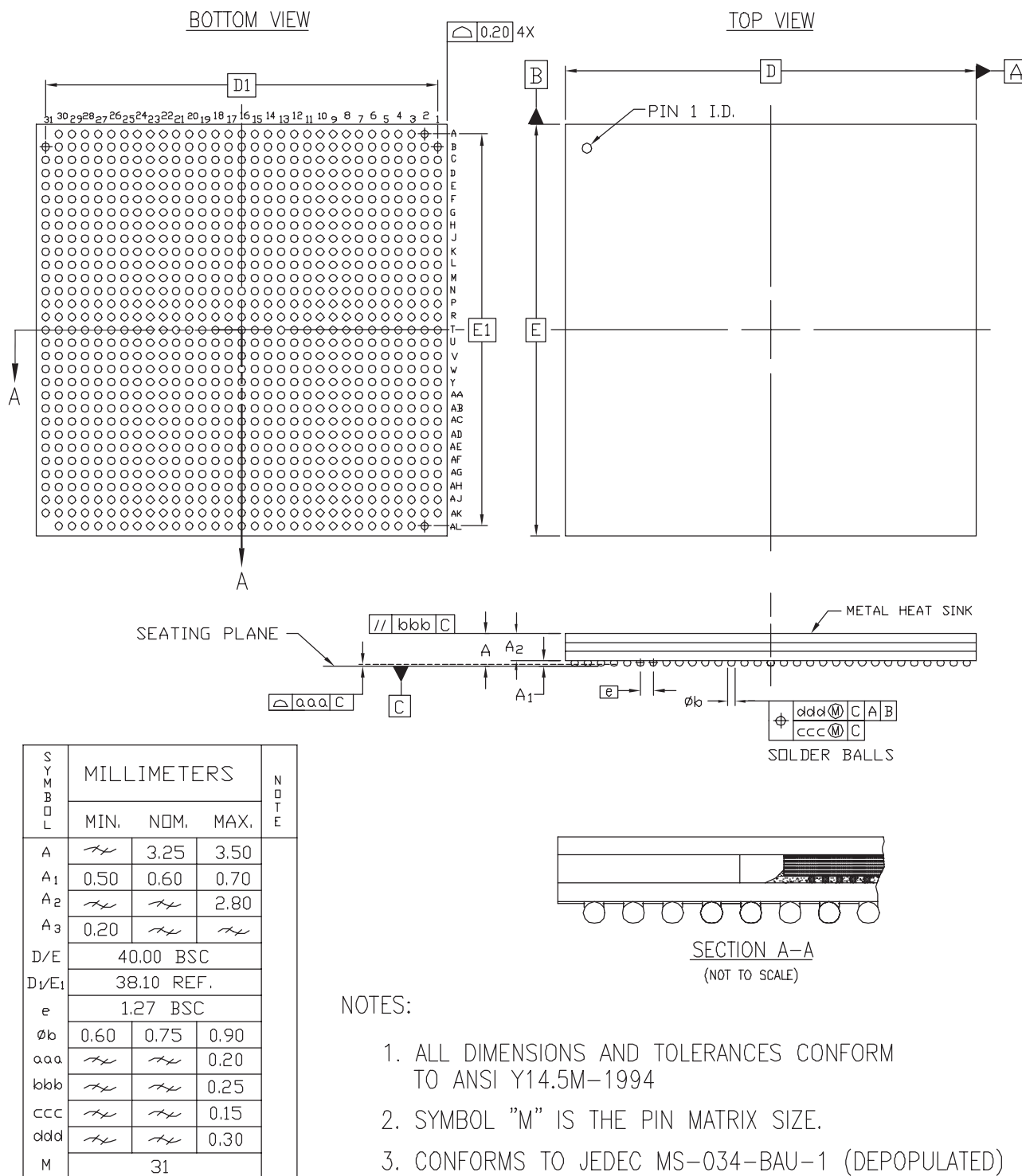
Figure 10: BF957 Flip-Chip BGA Package Specifications
