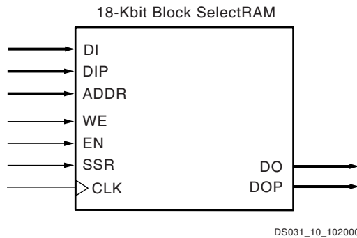
Figure 47: 18 Kb Block SelectRAM+ Memory in Single-Port Mode
