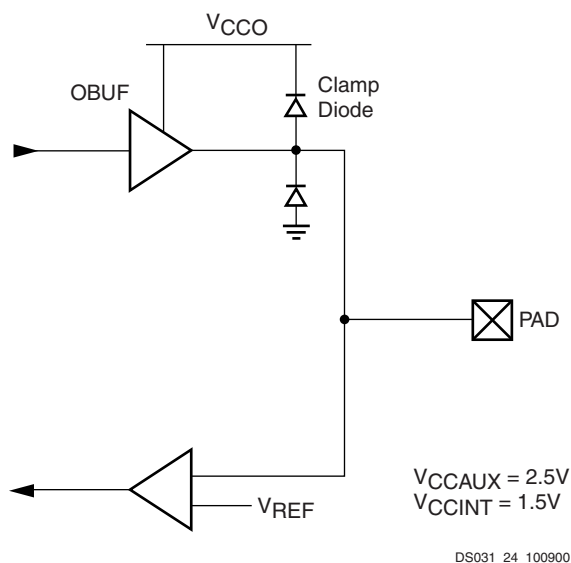
All pads are protected against damage from electrostatic discharge (ESD) and from over-voltage transients. Virtex-II Pro uses two memory cells to control the configuration of an I/O as an input. This is to reduce the probability of an I/O configured as an input from flipping to an output when subjected to a single event upset (SEU) in space applications.
