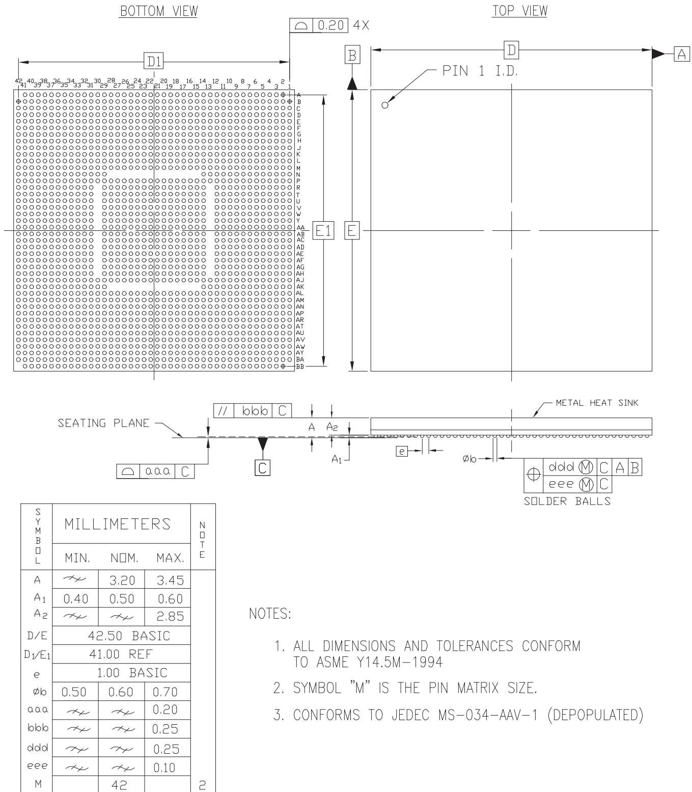
Figure 9: FF1704 Flip-Chip Fine-Pitch BGA Package Specifications
