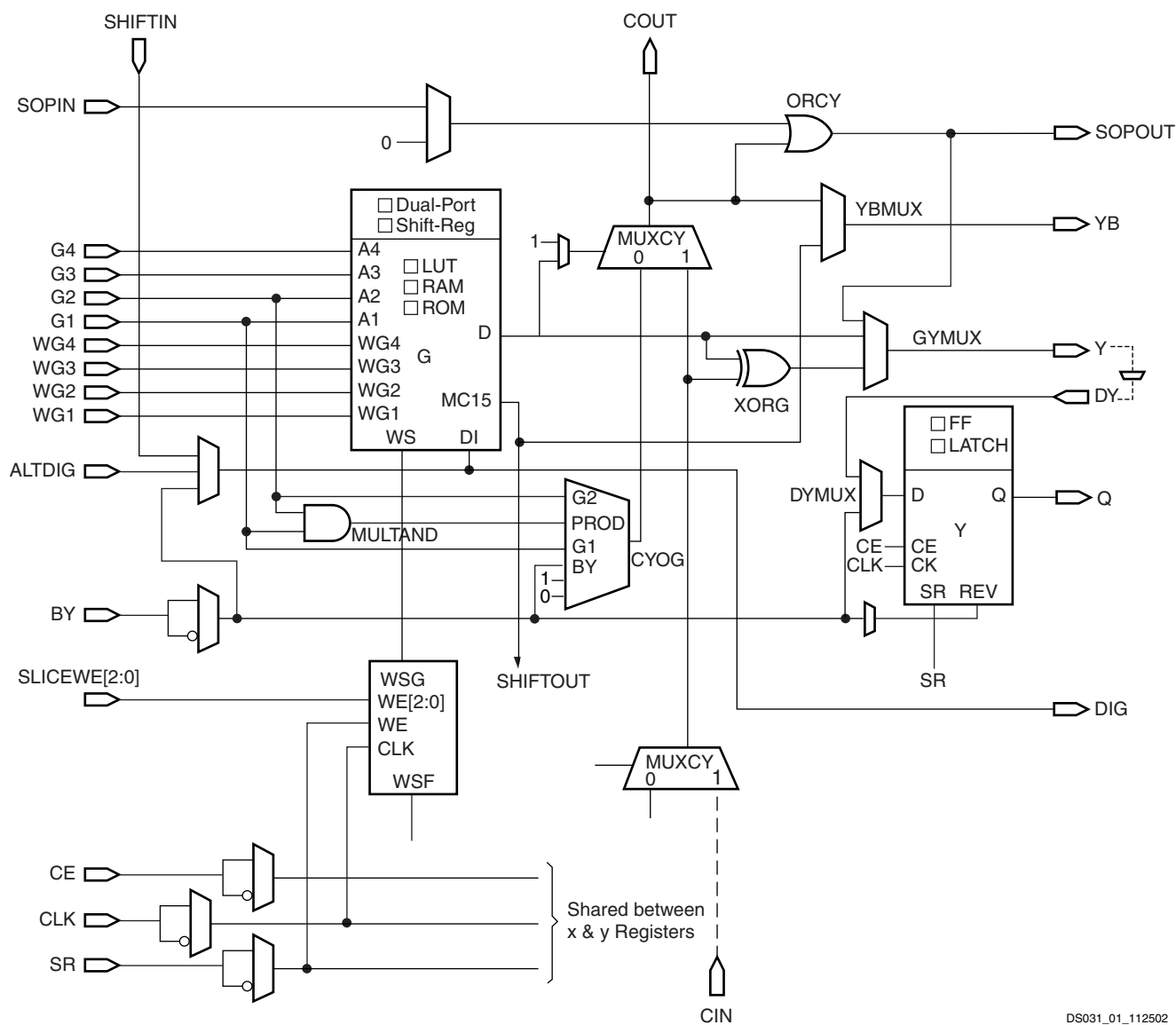
Figure 34: Virtex-II Pro Slice (Top Half)
