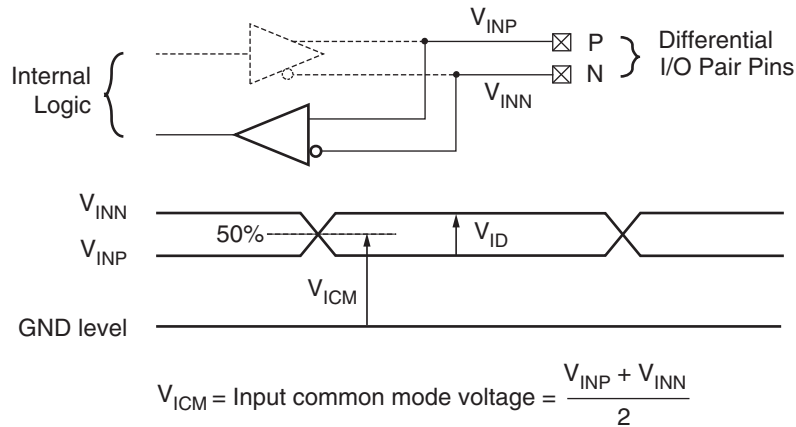
Figure 4: Differential Input Voltages
