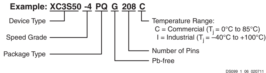
Figure 6: Pb-Free Packaging
