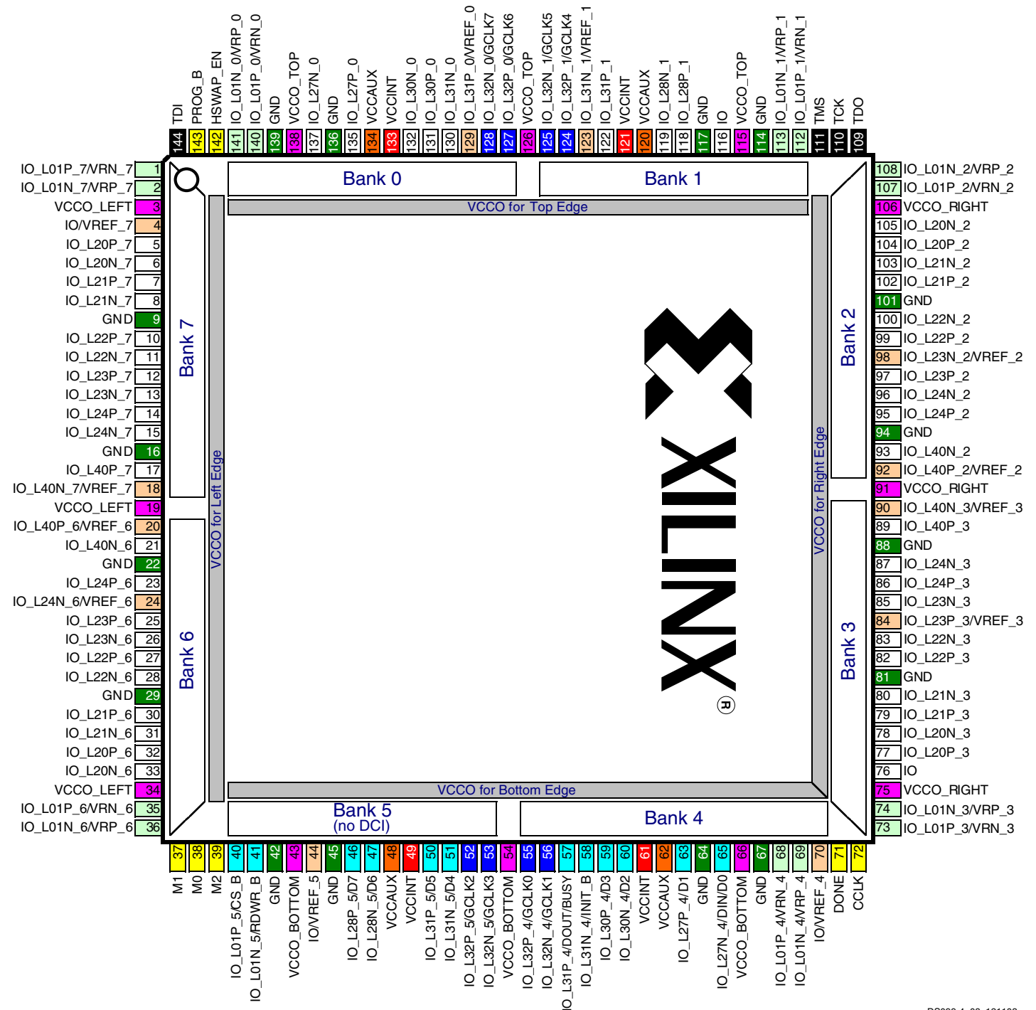
Figure 46: TQ144 Package Footprint (Top View). Note pin 1 indicator in top-left corner and logo orientation.
