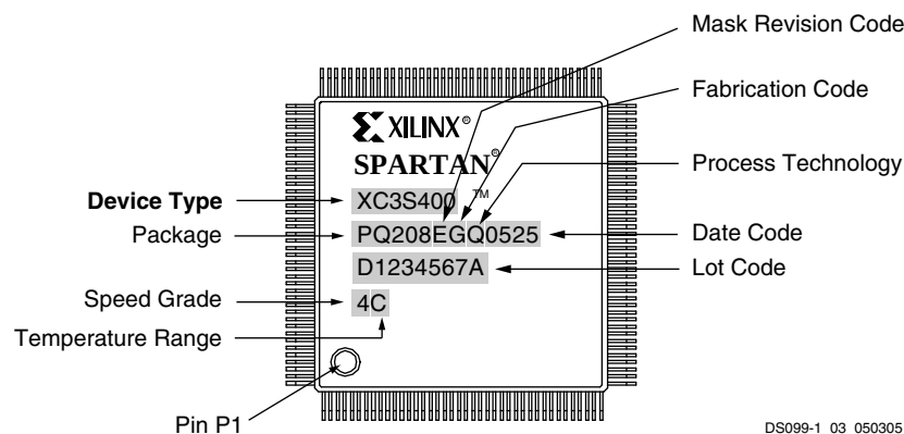
Figure 2: Spartan-3 FPGA QFP Package Marking Example for Part Number XC3S400-4PQG208C
