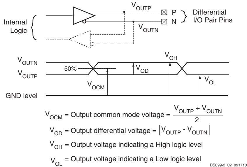
Figure 33: Differential Output Voltages
