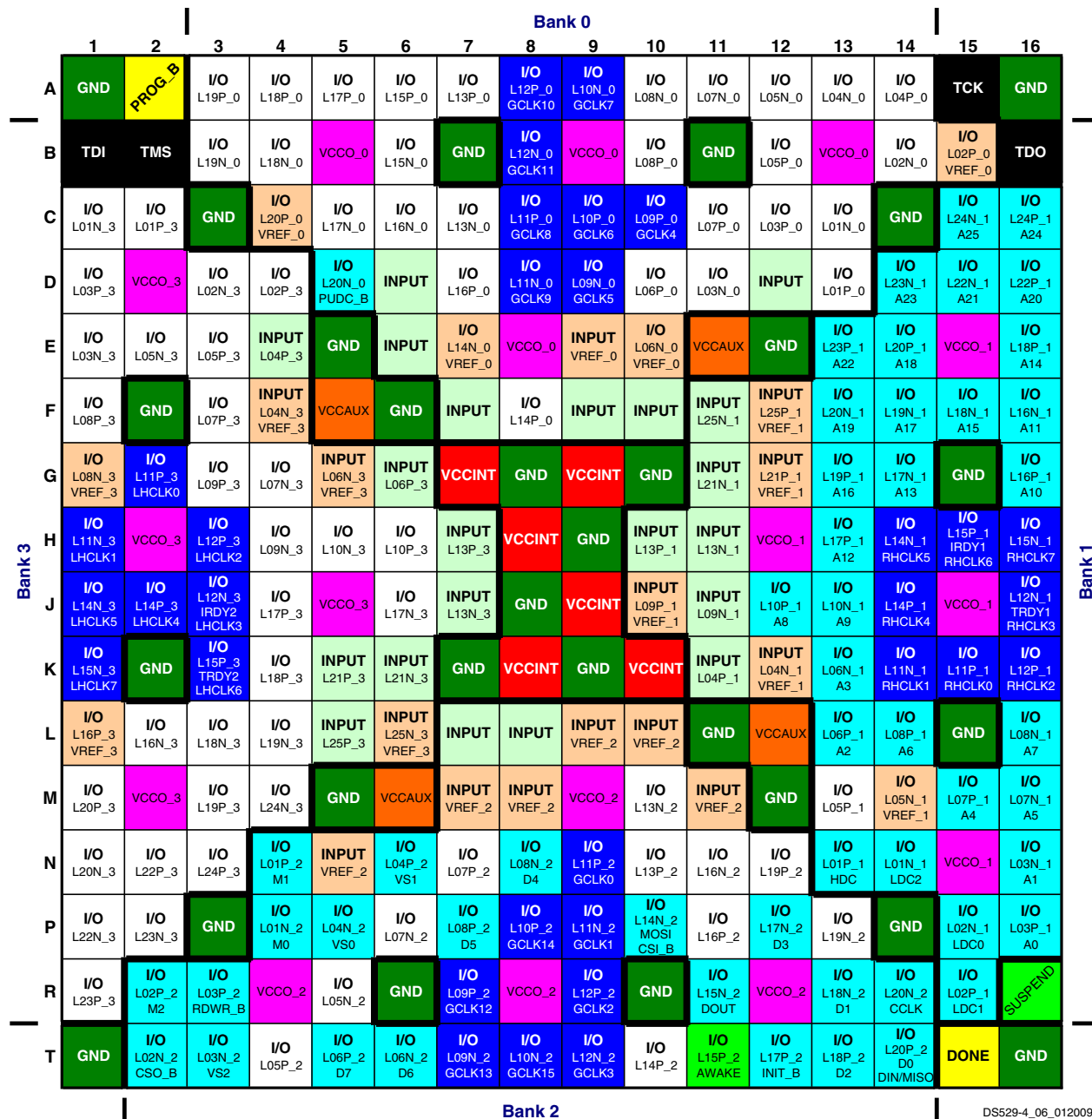
Figure 21: XC3S200A and XC3S400A FT256 Package Footprint (Top View)
