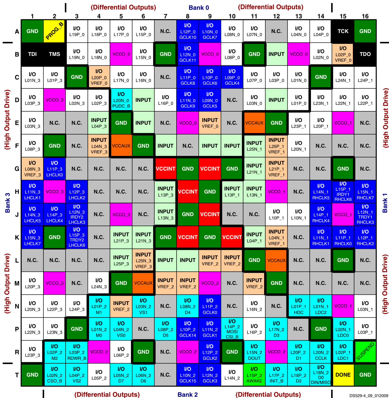
Figure 20: XC3S50A FT256 Package Footprint (Top View)
