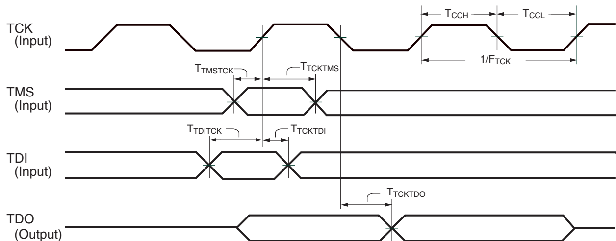
Figure 18: JTAG Waveforms
