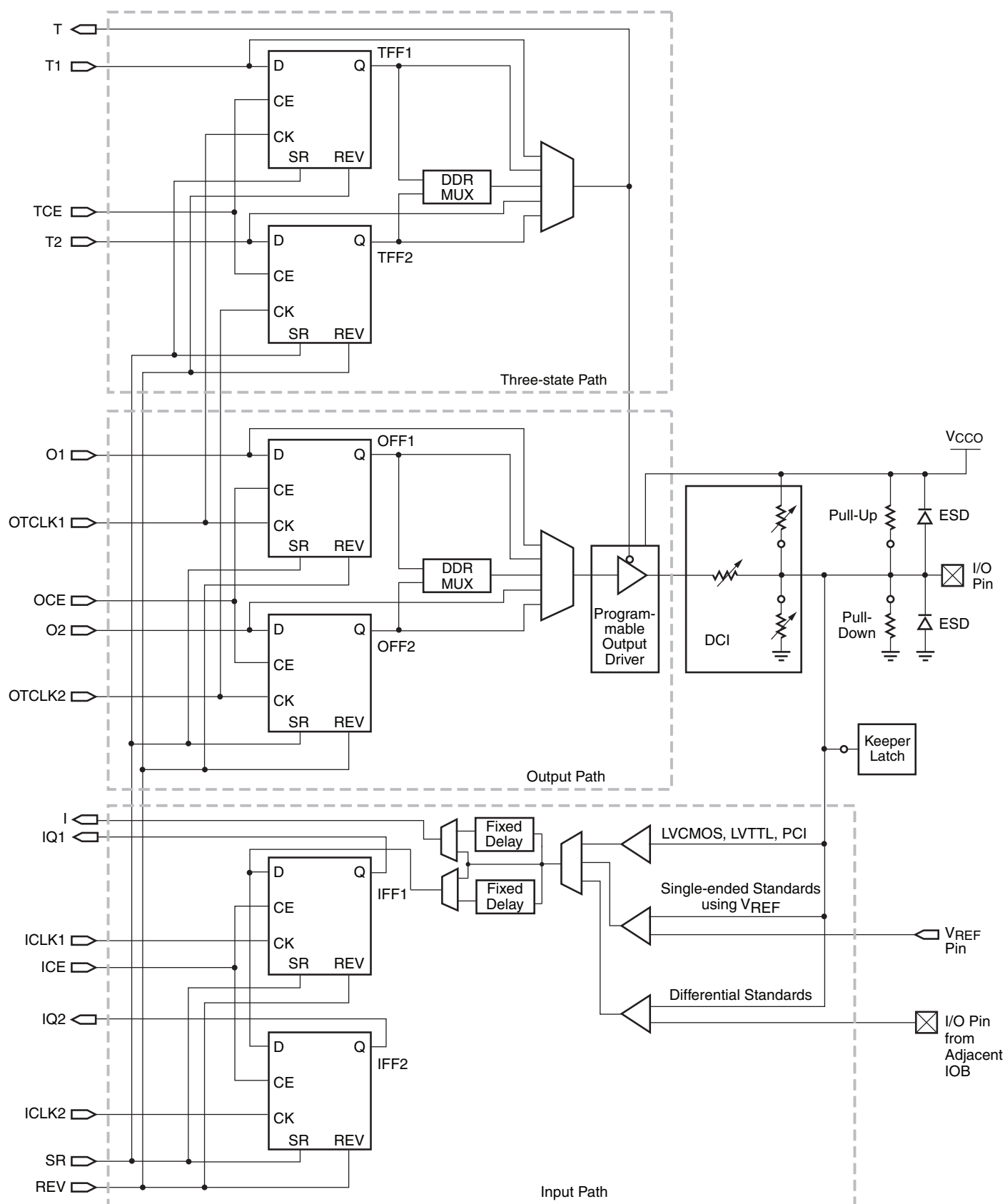
Figure 7: Simplified IOB Diagram
