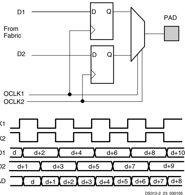
Figure 10: Output DDR
