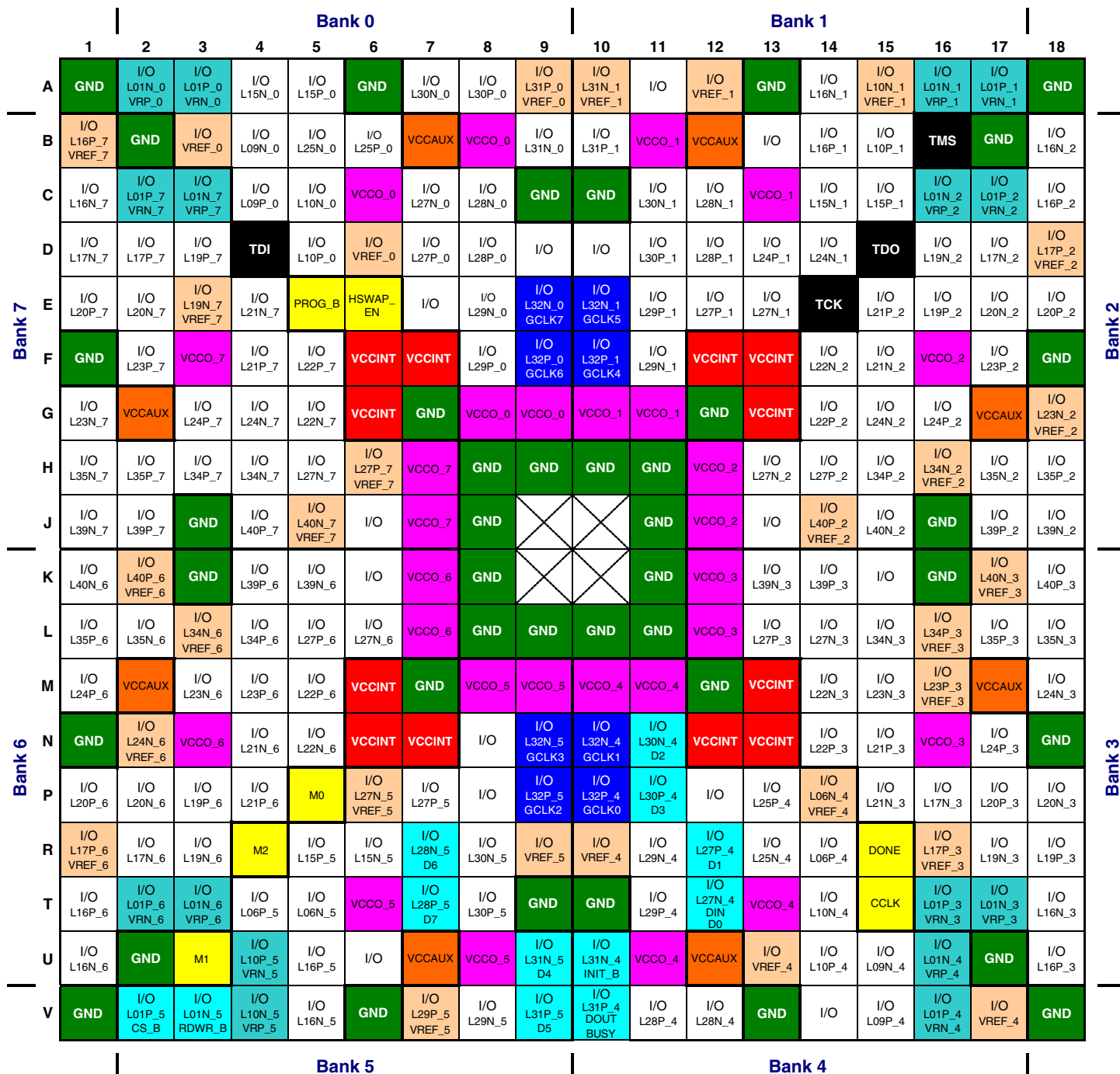
Figure 50: FG320 Package Footprint (Top View)
