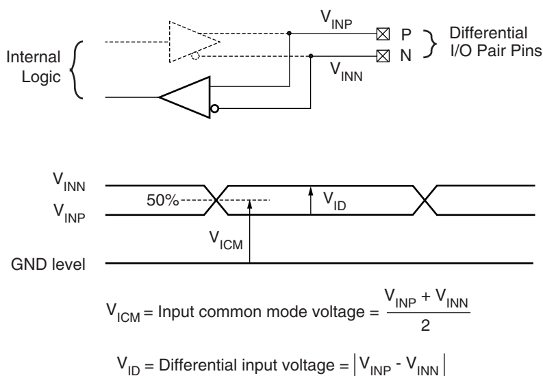
Figure 32: Differential Input Voltages
