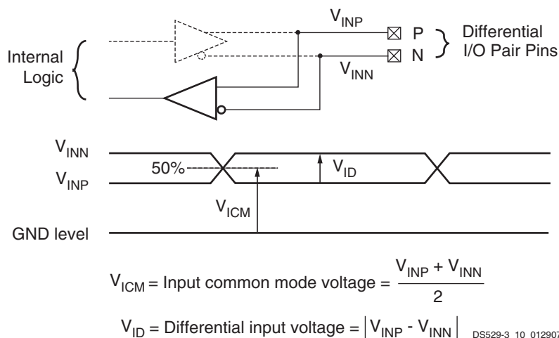
Figure 4: Differential Input Voltages
