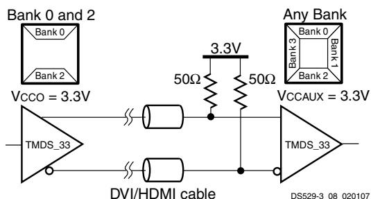
Figure 7: External Input Resistors Required for TMD5_33 I/O Standard
