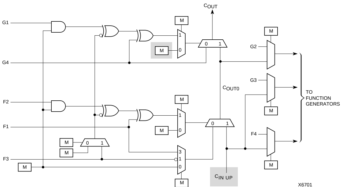
Figure 14: Detail of XC4000E Dedicated Carry Logic
