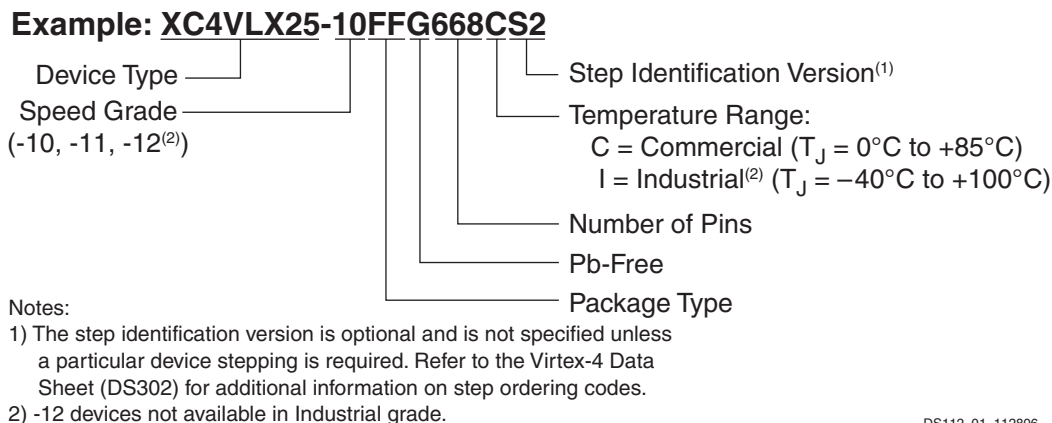
Figure 1: Virtex-4 FPGA Ordering Information
