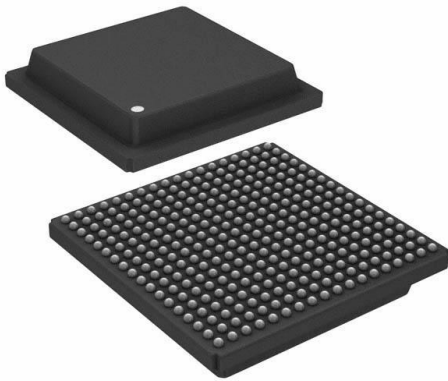
XC5VLX50-1FF324I
