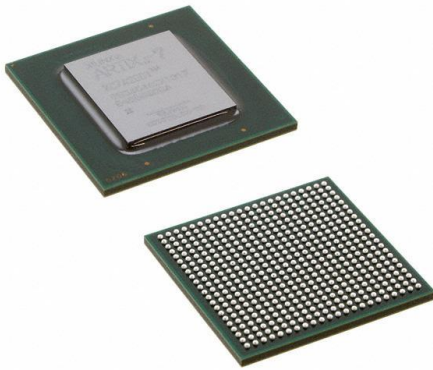
XC7A200T-1FBG676C
