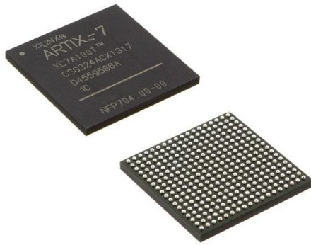
XC7A35T-L1CSG324I
