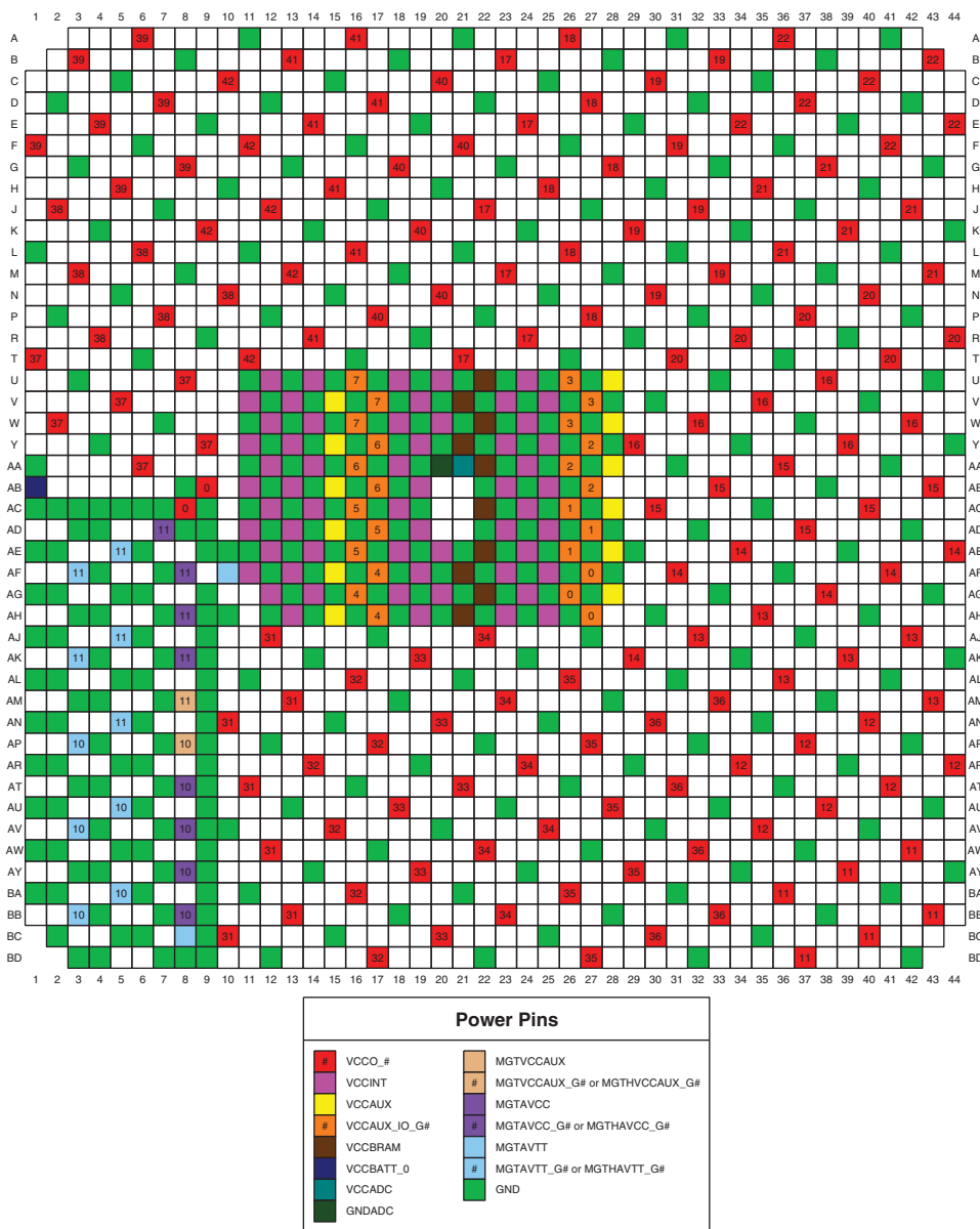
Figure 3-144: FL1925 and FLG1925 Packages—XC7V200T Power and GND Placement
