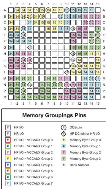
Figure 3-19: CSGA225 Package—XC7S25 and XA7S25 Memory Groupings
