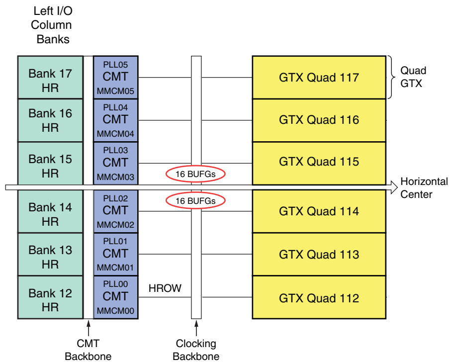
Figure 1-14: XC7K355T Banks
