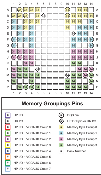
Figure 3-11: FTGB196 Package—XC7S25 and XC7S50 Memory Groupings
