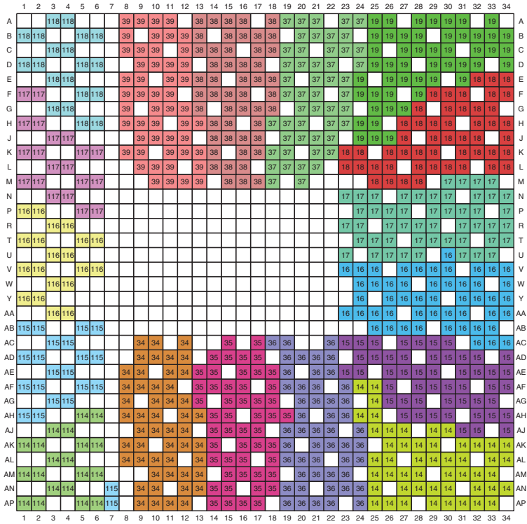
Figure 3-134: FF1157, FFG1157, and RF1157 Packages—XC7V585T I/O Banks
