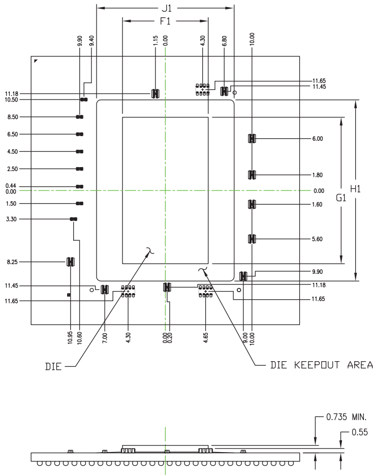
Figure 4-31: XC7K325T FB900, FBG900, and FBV900 Die Dimensions with Capacitor Locations
