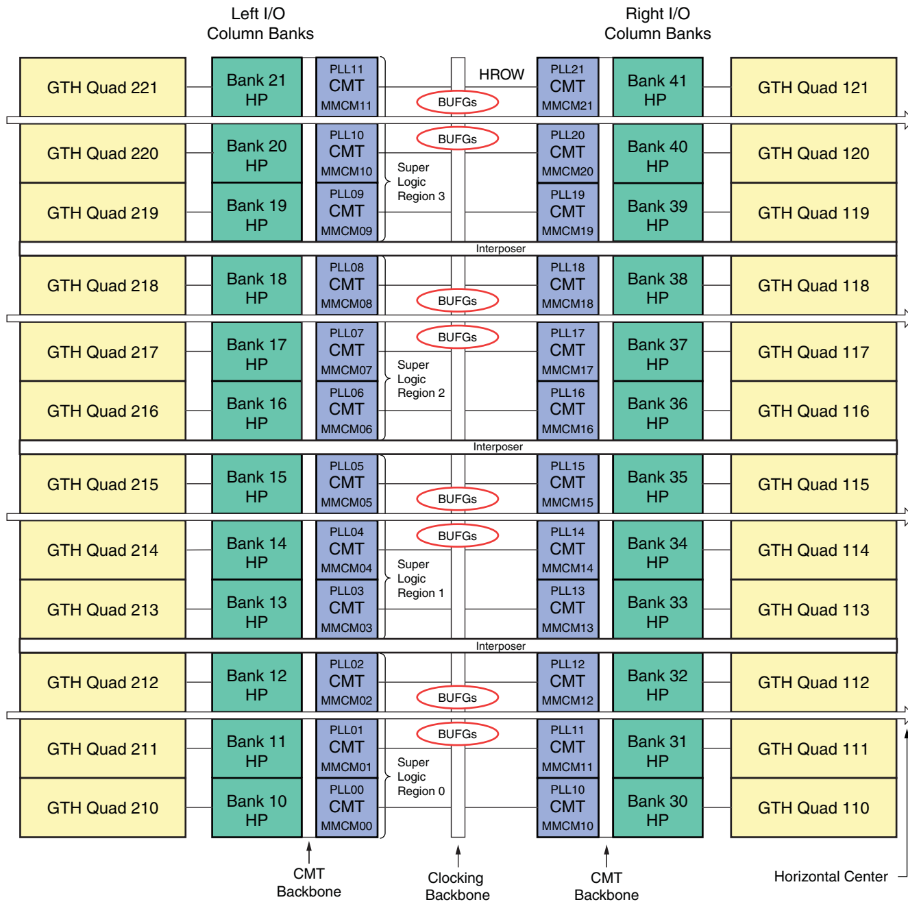
Figure 1-26: XC7VX1140T Banks
