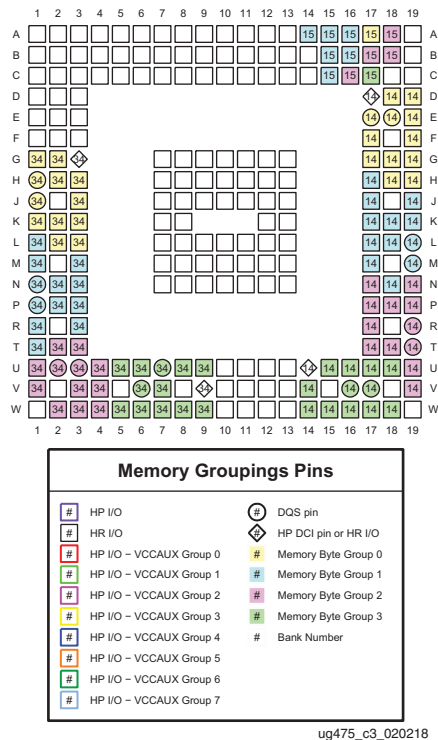
Figure 3-47: CPG238 Package—XC7A12T, XC7A25T, XA7A12T, and XA7A25T Memory Groupings
