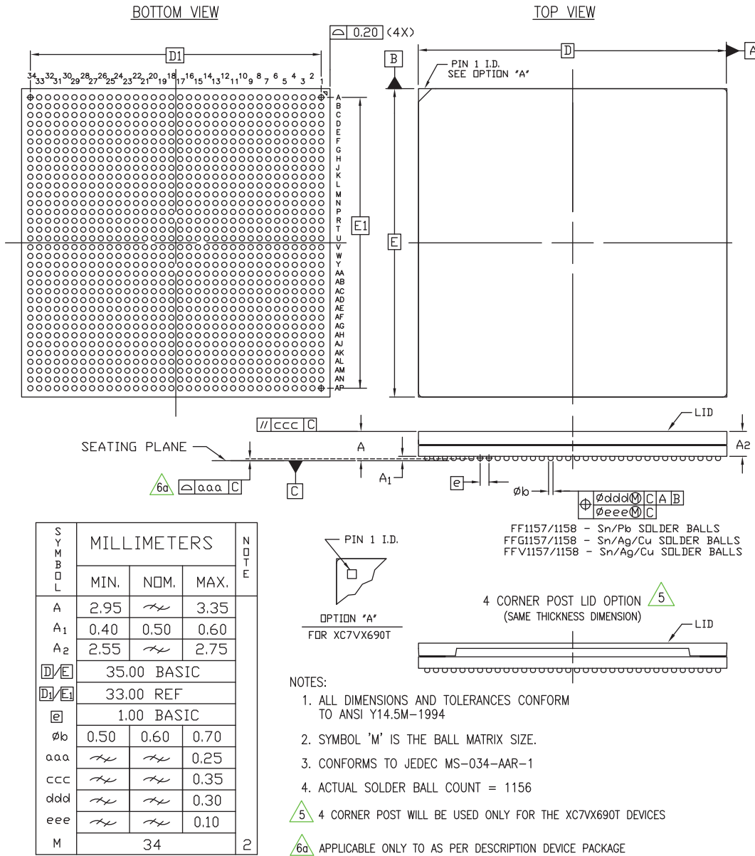
Figure 4-42: FF1157, FFG1157, FFV1157, FF1158, FFG1158, and FFV1158 Flip-Chip BGA Package Specification for XC7VX485T, XC7VX550T, XC7VX690T FPGAs
