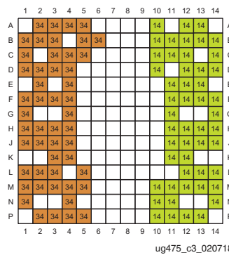
Figure 3-10: FTGB196 Package—XC7S25 and XC7S50 I/O Banks
