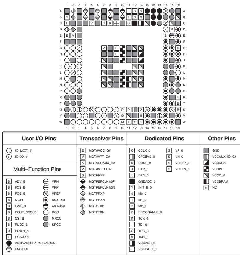
Figure 3-45: CPG238 Package—XC7A12T, XC7A25T, XA7A12T, and XA7A25T Pinout Diagram
