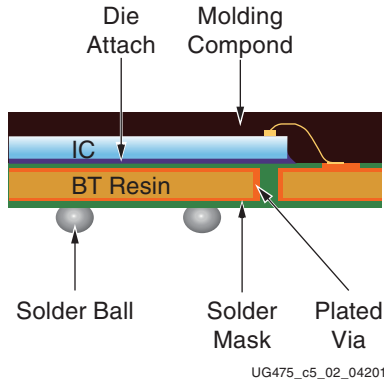
Figure 5-3: Rigid BT-Based Substrate Wire-Bond Packages
