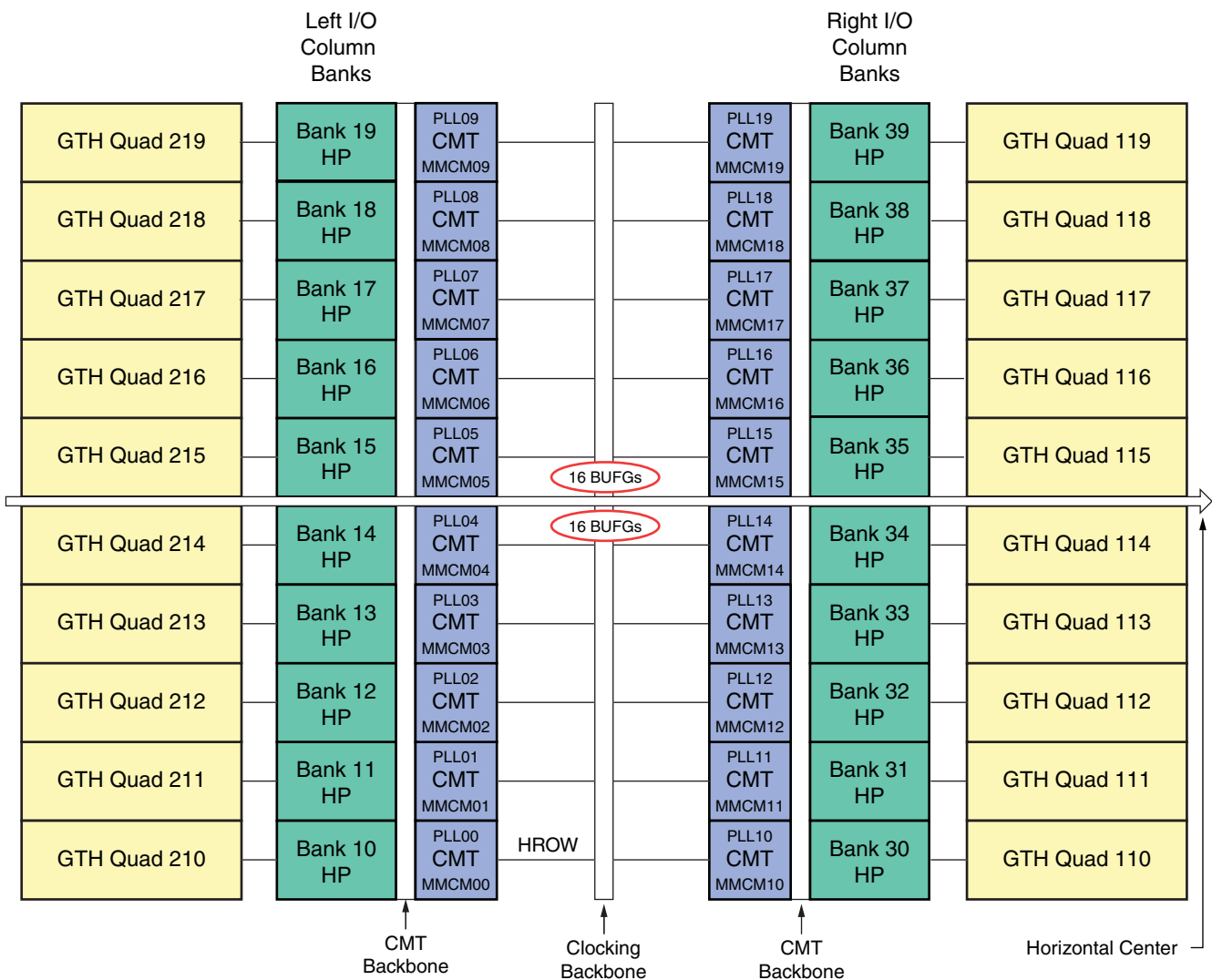
Figure 1-23: XC7VX550T Banks
