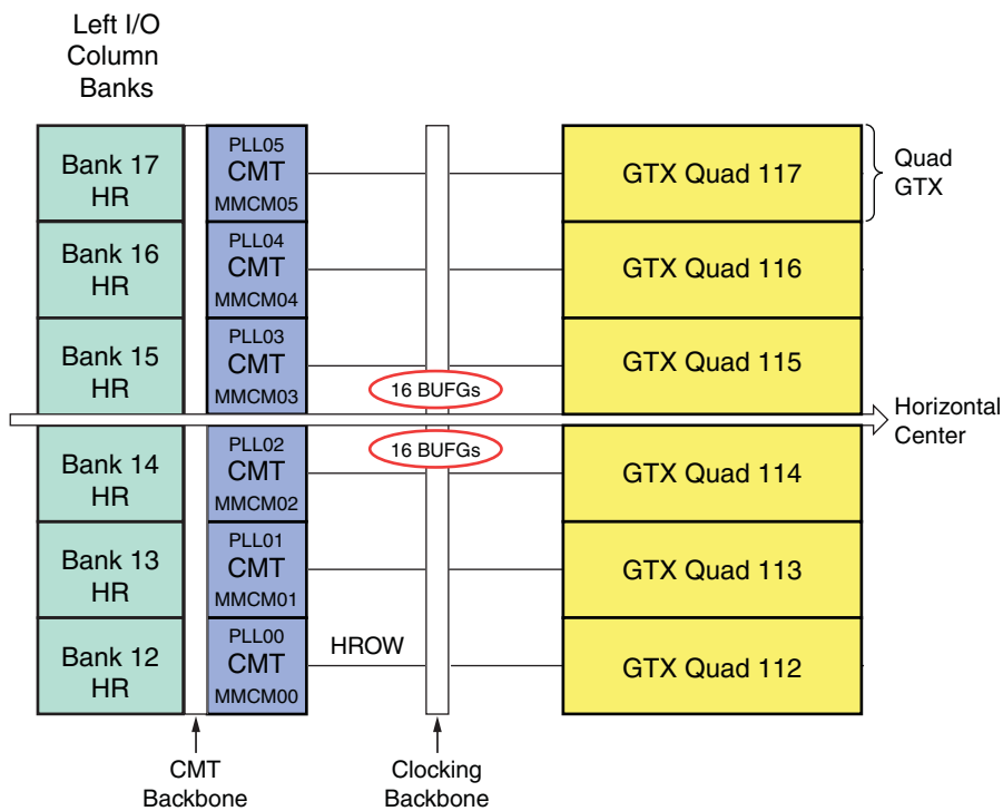
Figure 1-14: XC7K355T Banks
