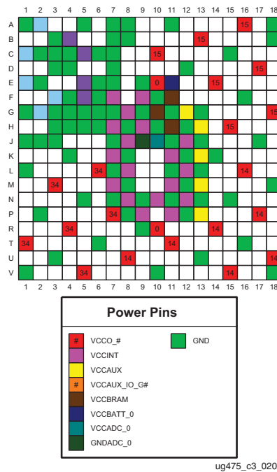
Figure 3-56: CSG325 Package—XC7A12T and XA7A12T Power and GND Placement
