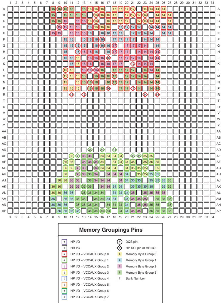
Figure 3-159: FF1158, FFG1158, FV1158, and RF1158 Packages—XC7VX415T, XC7VX550T, and XC7VX690T Memory Groupings
