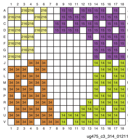
Figure 3-62: CS325 and CSG325 Packages—XC7A15T, XC7A35T, and XC7A50T CSG325 Packages (only)—XA7A15T, XA7A35T, and XA7A50T I/O Banks
