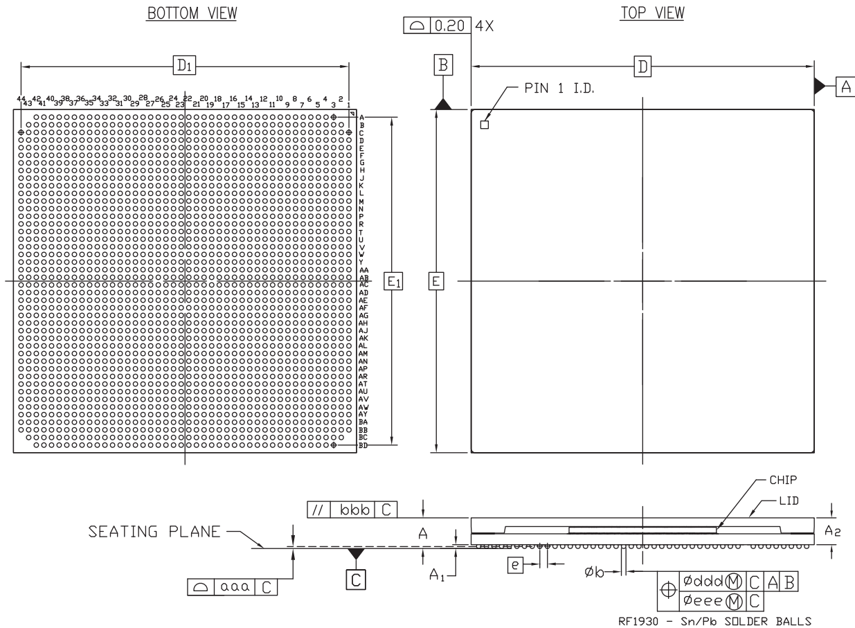
RF1930 - Sn/Pb SOLDER BALLS
