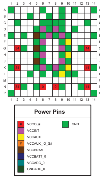
Figure 3-8: FTGB196 Package—XC7S6 and XC7S15 Power and GND Placement
