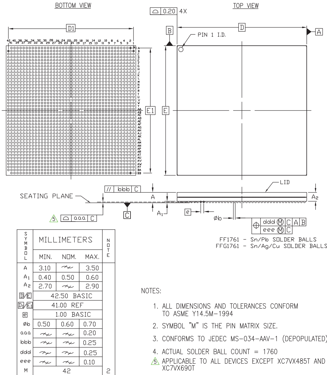
Figure 4-44: FF1761 and FFG1761 Flip-Chip BGA Package Specification for XC7V585T and XC7VX330T FPGAs
