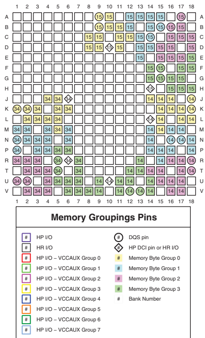
Figure 3-63: CS325 and CSG325 Packages—XC7A15T, XC7A35T, and XC7A50T CSG325 Packages (only)—XA7A15T, XA7A35T, and XA7A50T Memory Groupings
