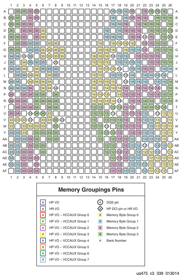
Figure 3-91: FB676, FBG676, FBV676, and RB676 Packages—XC7A200T Memory Groupings
