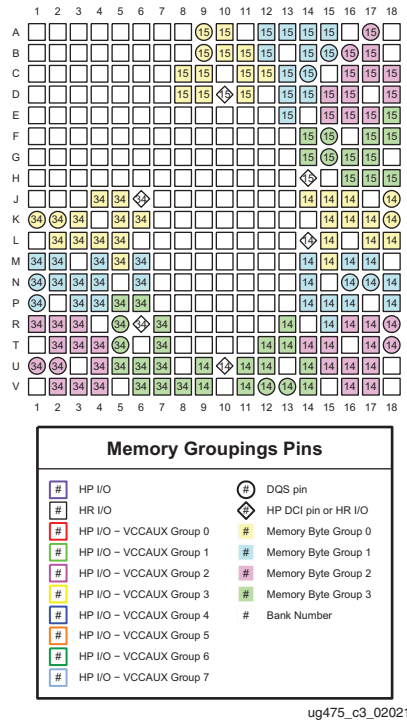
Figure 3-55: CSG325 Package—XC7A12T and XA7A12T Memory Groupings
