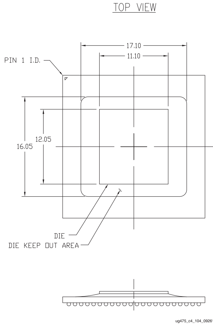
Figure 4-13: XC7A200T FB484, FBG484, and FBV484 Die Dimensions
