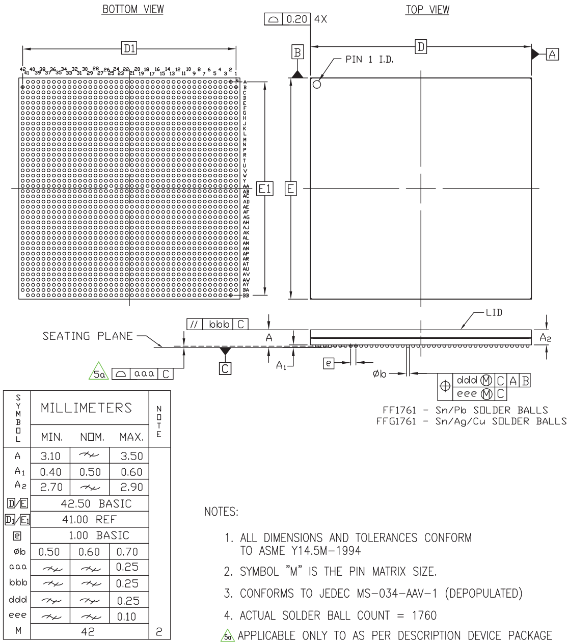
Figure 4-43: FF1761 and FFG1761 Flip-Chip BGA Package Specification for XC7VX485T and XC7VX690T FPGAs
