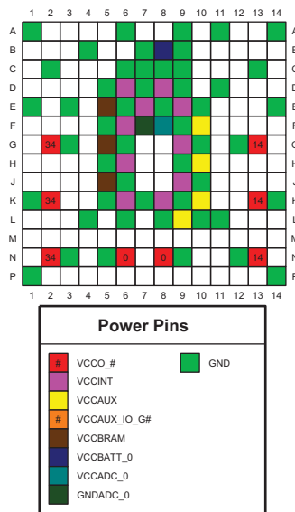
Figure 3-12: FTGB196 Package—XC7S25 and XC7S50 Power and GND Placement
