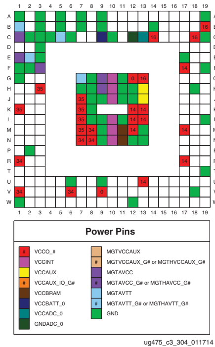
Figure 3-44: CP236 and CPG236 Packages—XC7A15T, XC7A35T, and XC7A50T CPG236 Packages (only)—XA7A15T, XA7A35T, and XA7A50T Power and GND Placement
