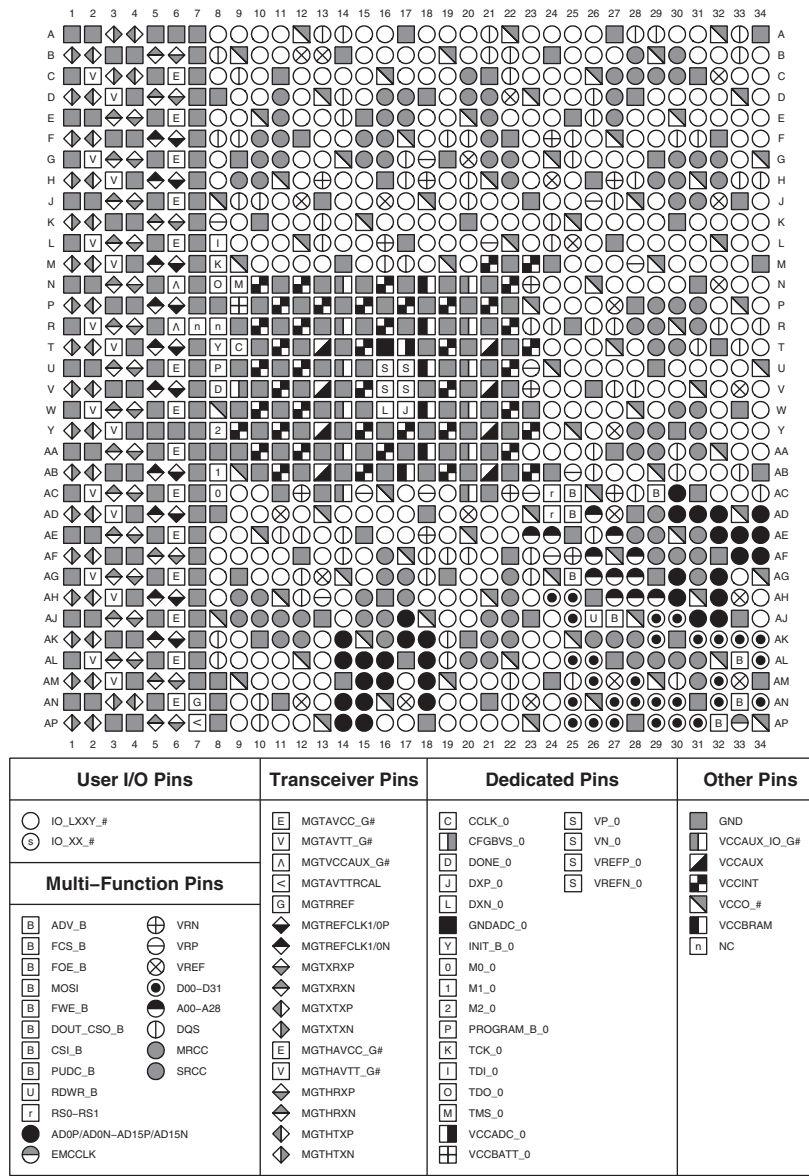
Figure 3-149: FF1157, FFG1157, and RF1157 Packages—XC7VX330T, XC7VX415T, and XC7VX690T Pinout Diagram
