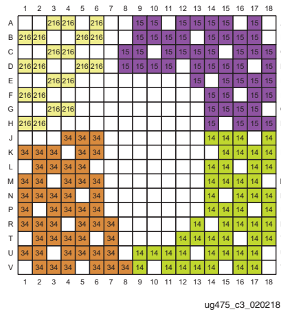
Figure 3-58: CSG325 Package—XC7A25T and XA7A25T I/O Banks
