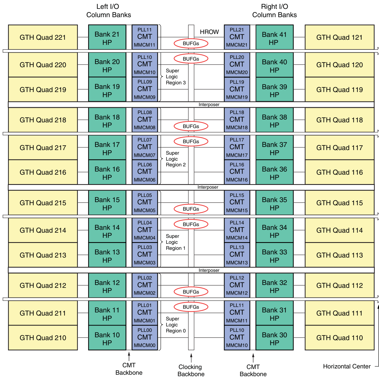
Figure 1-26: XC7VX1140T Banks
