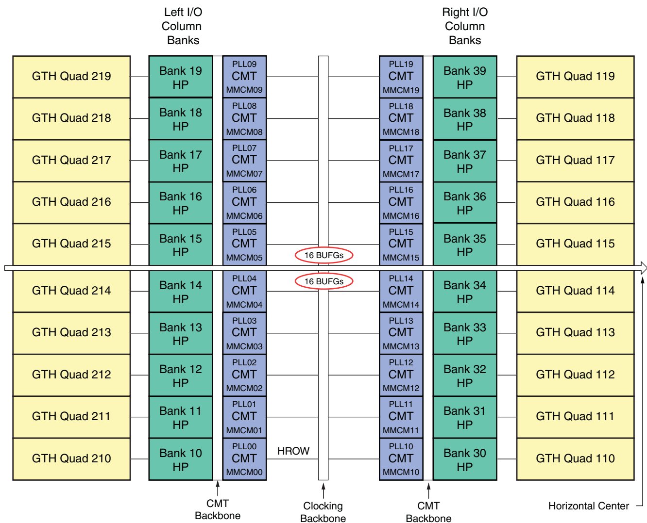
Figure 1-23: XC7VX550T Banks
