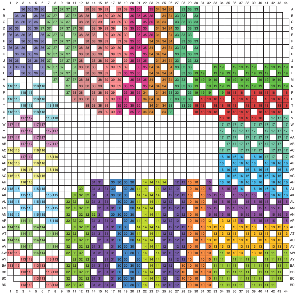
Figure 3-198: FF1930, FFG1930, and RF1930 Packages—XC7VX690T I/O Banks
