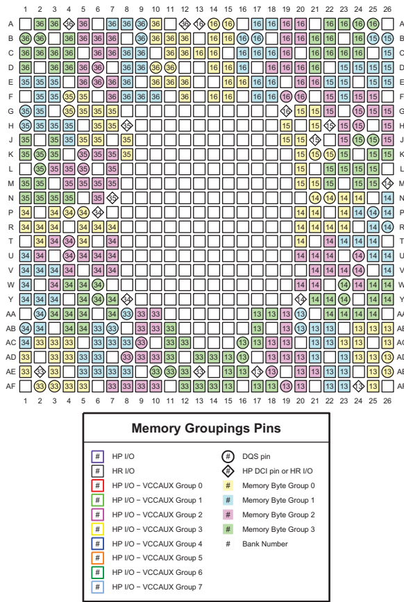
Figure 3-39: FGGA676 Package—XC7S75, XC7S100, XA7S75, and XA7S100 Memory Groupings
