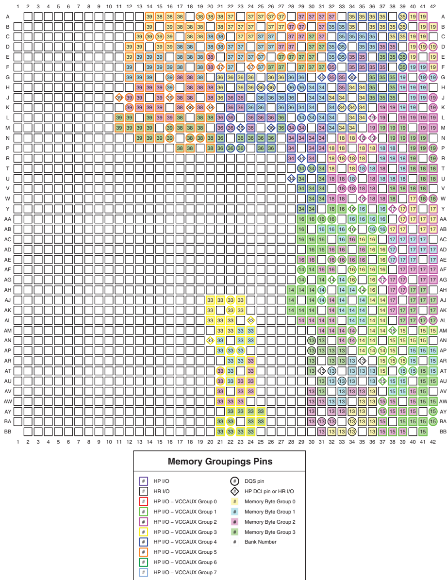
Figure 3-155: FF1761, FFG1761, and RF1761 Packages—XC7VX330T Memory Groupings
