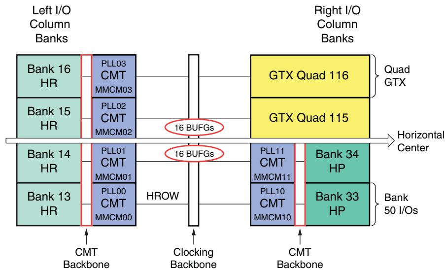
Figure 1-11: XC7K70T Banks
