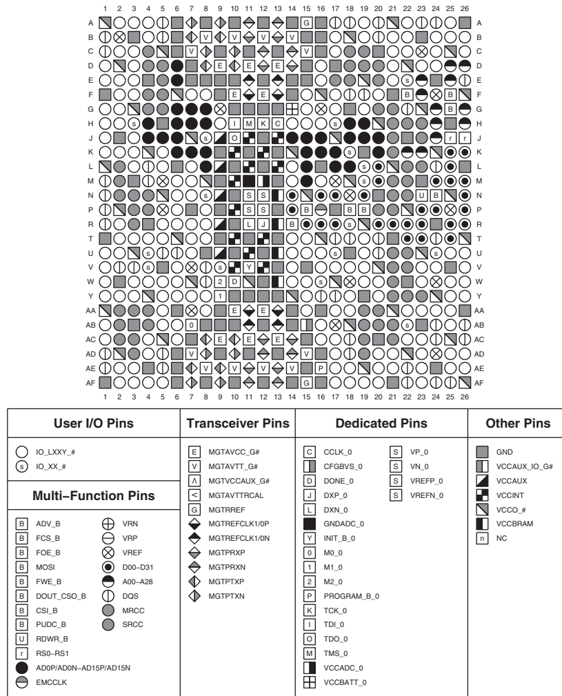
Figure 3-89: FB676, FBG676, FBV676, and RB676 Packages—XC7A200T Pinout Diagram
