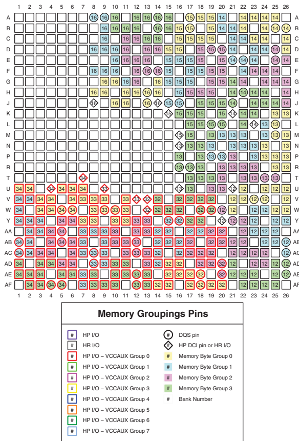
Figure 3-115: FF676, FFG676, FFV676, and RF676 Packages—XC7K160T, XA7K160T, XC7K325T, and XC7K410T Memory Groupings
