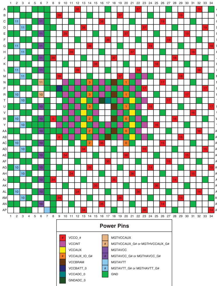
Figure 3-168: FF1157, FFG1157, and FFV1157 Packages—XC7VX485T Power and GND Placement
