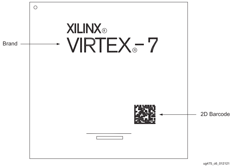
Figure 6-9: Virtex 7 Device Package Marking with Simplified 2D Bar Code
