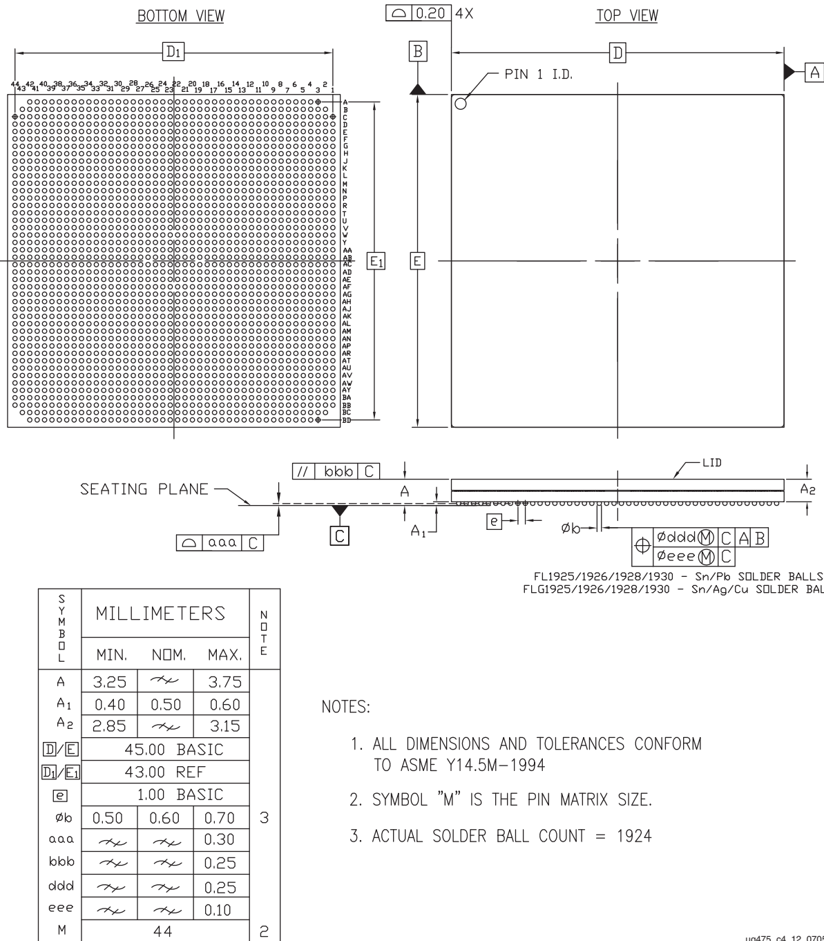
Figure 4-49: FL1925, FLG1925, FL1926, FLG1926, FL1928, FLG1928, and FL1930, FLG1930 Flip-Chip BGA Package Specification for Virtex 7 FPGAs
