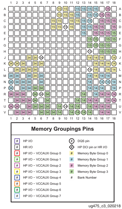
Figure 3-59: CSG325 Package—XC7A25T and XA7A25T Memory Groupings
