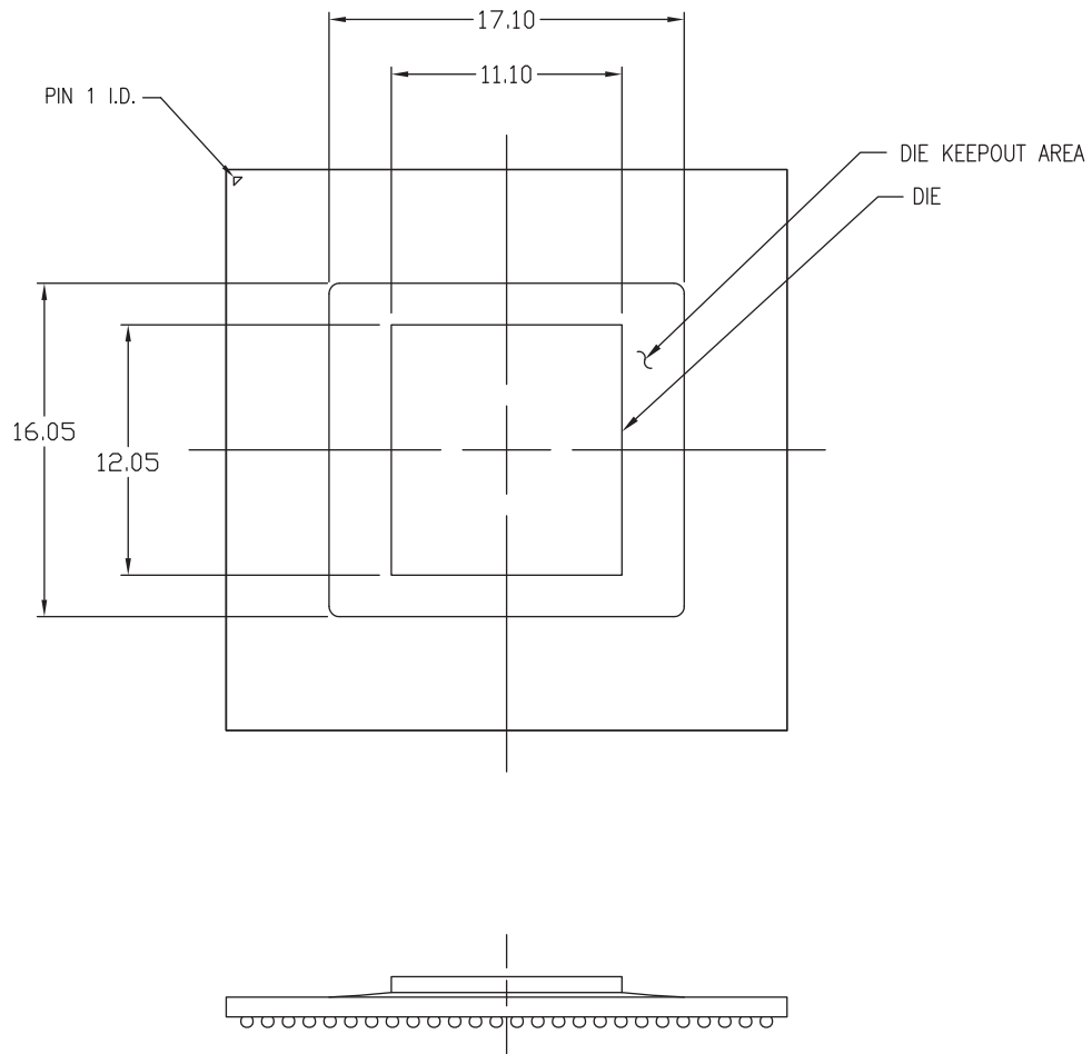
Figure 4-15: XC7A200T FB676, FBG676, and FBV676 Die Dimensions
