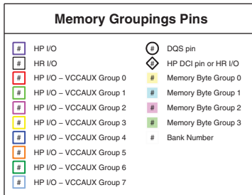
Figure 3-139: FF1761, FFG1761, and RF1761 Packages—XC7V585T Memory Groupings
