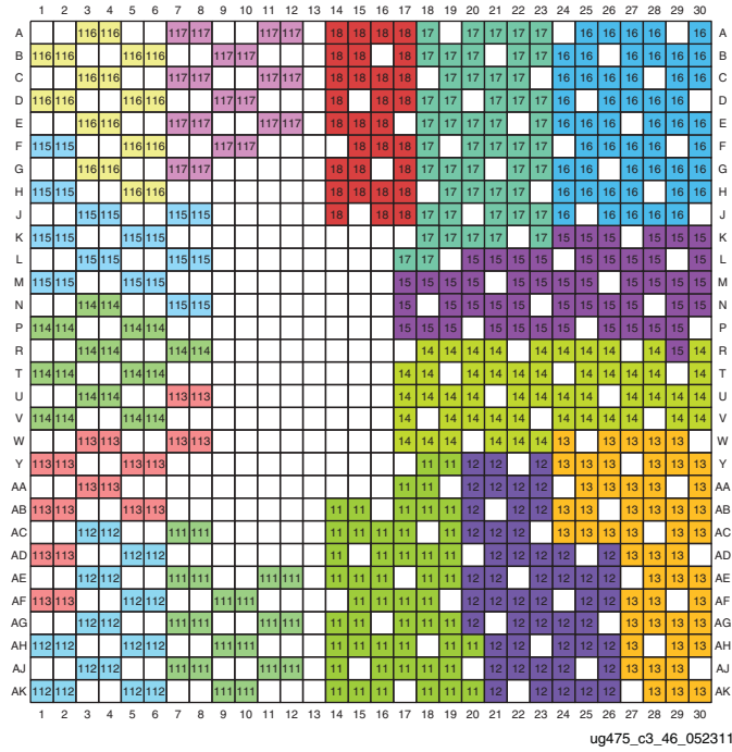
Figure 3-126: FF901, FFG901, and FFV901 Packages—XC7K420T and XC7K480T I/O Banks
