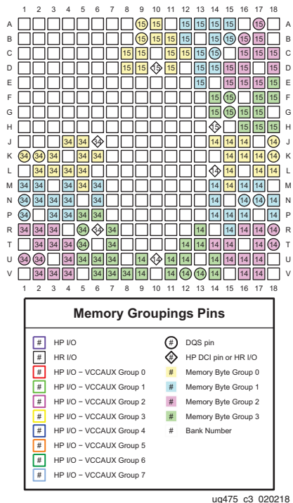
Figure 3-59: CSG325 Package—XC7A25T and XA7A25T Memory Groupings
