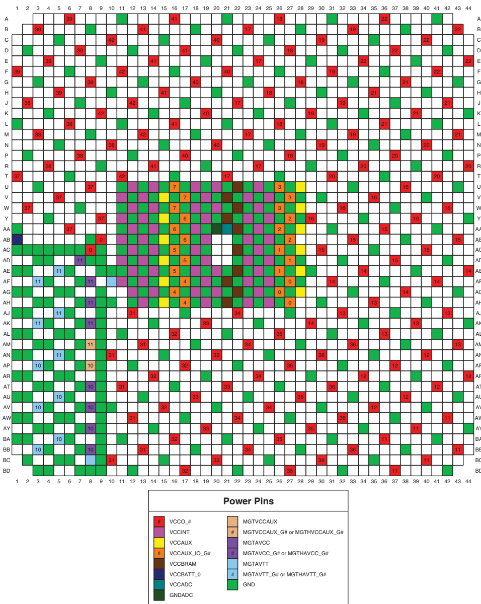
Figure 3-144: FL1925 and FLG1925 Packages—XC7V2000T Power and GND Placement
