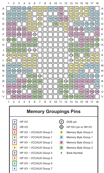
Figure 3-27: CSGA324 Package—XC7S50 and XA7S50 Memory Groupings
