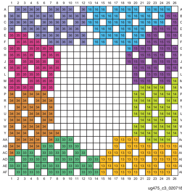
Figure 3-38: FGGA676 Package—I/O Banks—XC7S75, XC7S100, XA7S75, and XA7S100 I/O Banks
