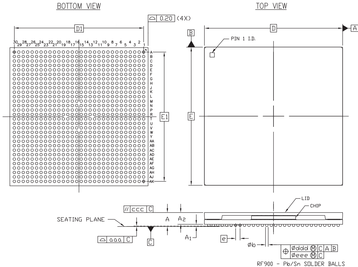
RF900 - Pb/Sn SOLDER BALLS
