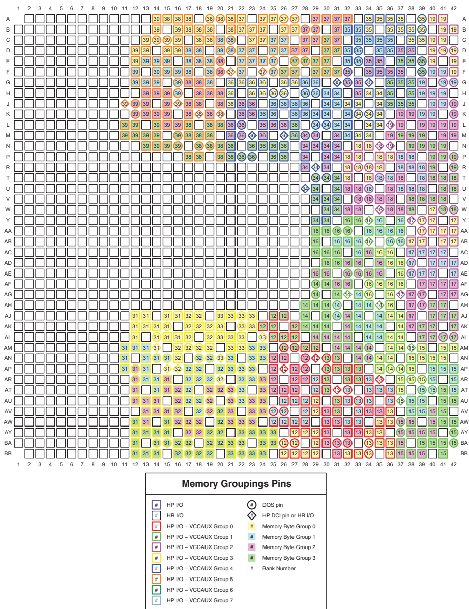
Figure 3-187: FF1761, FFG1761, and RF1761 Packages—XC7VX690T Memory Groupings
