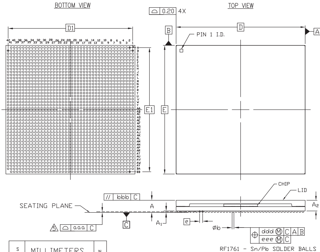
RF1761 - Sn/Pb SOLDER BALLS
