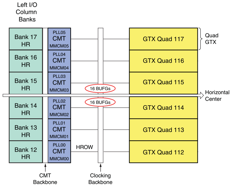
Figure 1-14: XC7K355T Banks
