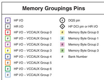
Figure 3-139: FF1761, FFG1761, and RF1761 Packages—XC7V585T Memory Groupings
