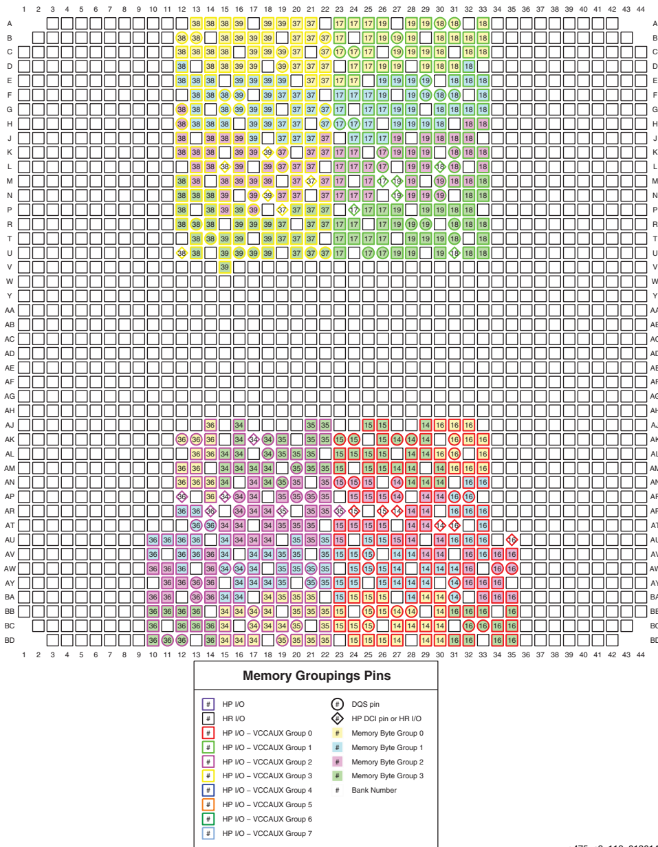
Figure 3-163: FF1927, FFG1927, and FV1927 Packages—XC7VX415T Memory Groupings
