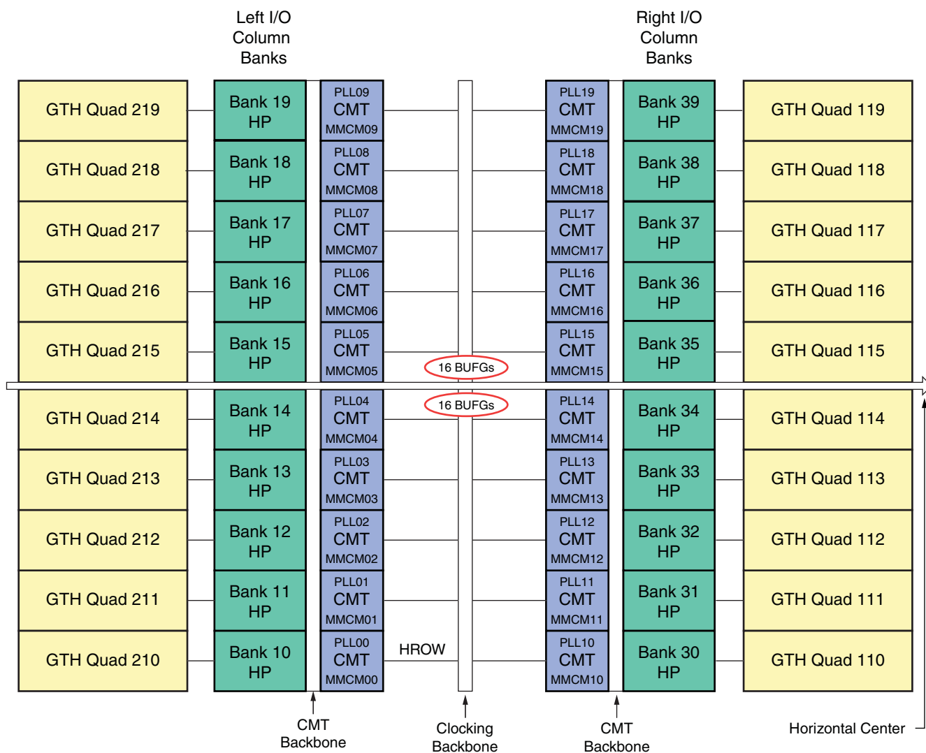
Figure 1-23: XC7VX550T Banks
