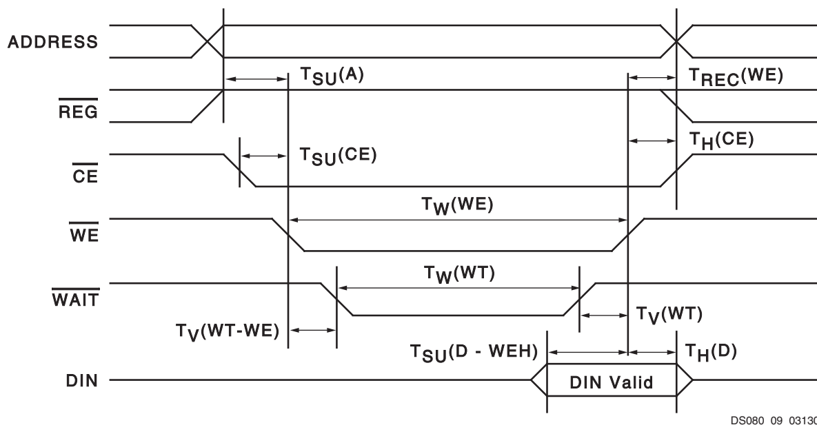
Figure 6: CompactFlash Common Memory Write Timing Diagram
